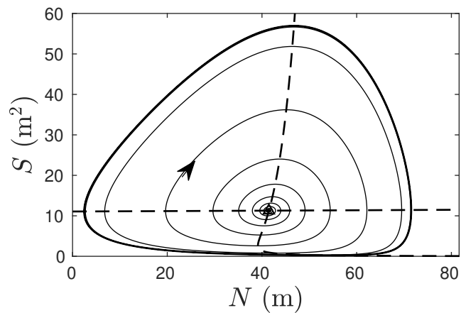
Figure 4. The periodic solution of figure 3 plotted in a phase plane. The thin curve represents a solution that approaches the limit cycle shown as a by the thick curve as indicated by the arrow. The instability of the steady state solution (where the nullclines cross) is clearly visible, since evolution along the thin line is away from that steady state.
