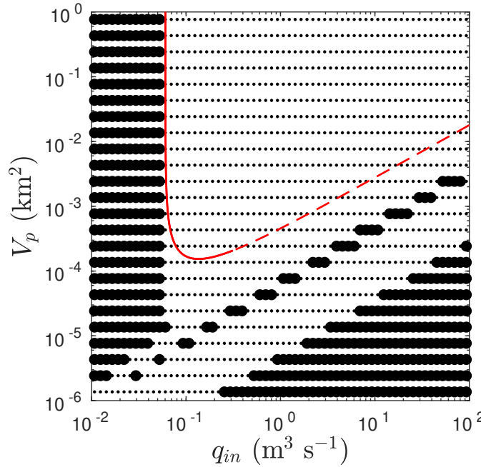
Figure 12. Stability boundary plotted in the same way as in figure 2, but with \Psi_0 = 1630 \text{ Pa m}^{-1} , u_b h_r = 1.05 \times 10^{-07} \text{ m}^2 \text{ s}^{-1} , and we put L=5000 L=10000 m.
