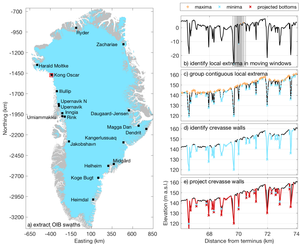
520 Figure 1: Map of glacier locations and example of the crevasse depth estimation approach applied to the elevation data for each glacier. a) Operation IceBridge transects (black squares) overlain on the Greenland Ice Mapping Project ice mask (light blue) and land mask (gray). Glacier names are from Bjork et al. (2015). The red box highlights the location of the profile in panels b-e. b) Moving window approach to find local extrema. The nested search windows (gray shading) and local extrema (colored points) overlain on the de-trended portion of the profile. Local extrema (blue dots) were filtered to c) isolate crevasse bottoms (blue x's) and top edges (orange +'s), d) locate steeply-sloped crevasse walls (blue lines), and e) project wall slopes to depth. 525
