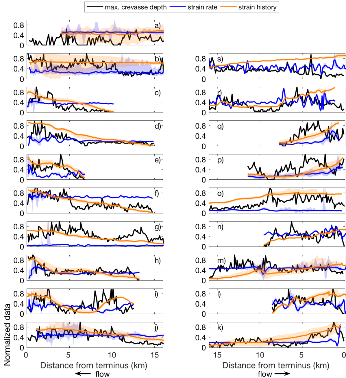
540 Figure 3: Normalized profiles of maximum crevasse depth, local strain rate, and strain history. In each panel, the maximum crevasse depth in 150 m-wide bins is in black, the local strain rate is in blue, and the strain history is in orange. The median strain rate and strain history are shown as lines with shading indicating their temporal ranges. As in Fig. 2, the panels are geographically arranged.
