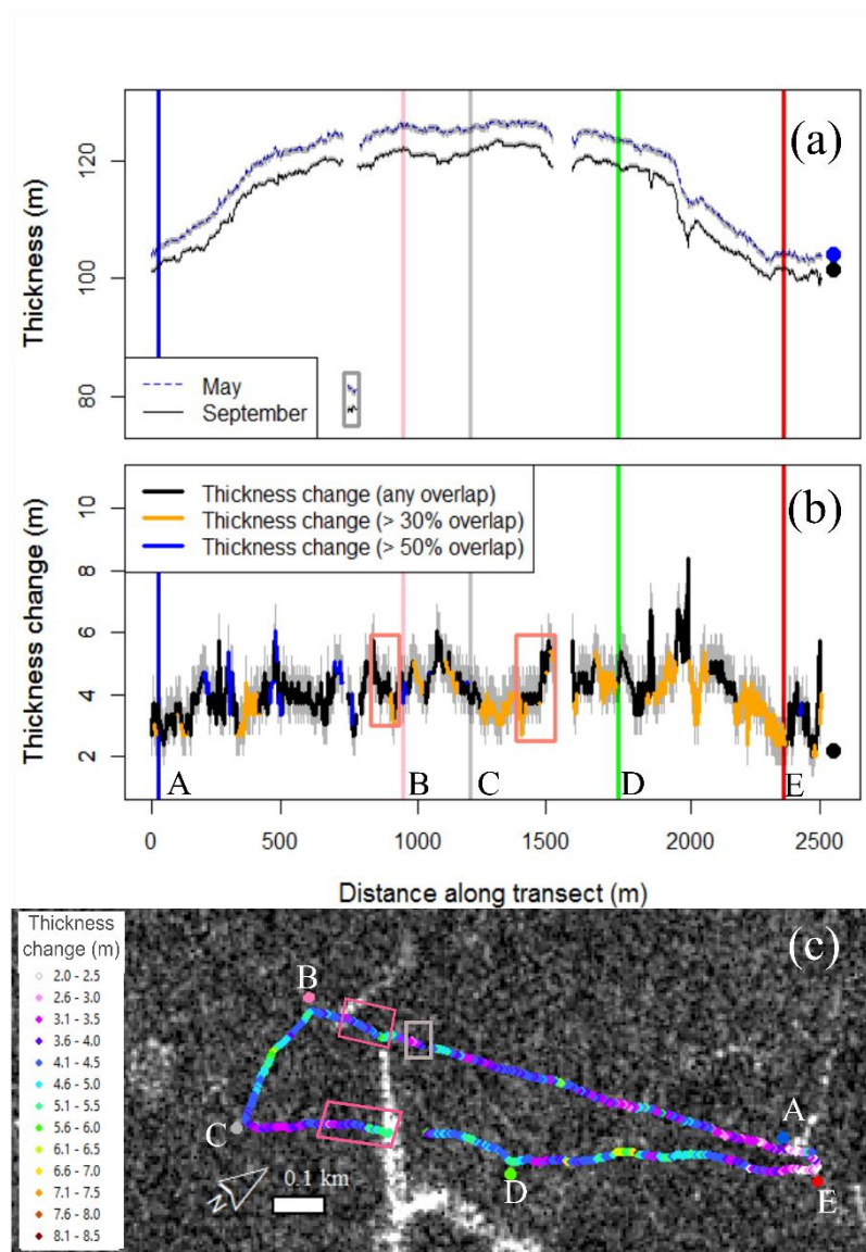
Figure 5: Spatial variation in morphology and thinning between May and September 2016. Upper-case letters are used to denote transect segments referred to in the text. (a) Thickness observations collected with mobile ice penetrating radar. The grey box corresponds with the thin ice section also denoted in (c). (b) Thickness change. The pink boxes indicate thickness change gradients also identified in (c). Thinning data were categorized based on the amount of overlap between the May and September radar footprints. Grey shading in (a) and (b) denotes uncertainty in thickness measurements and thinning amounts, respectively. The larger, single points denote the respective thickness and thinning measured with corresponding data collected by the sIPR at the main site. (c) Thickness change displayed on a Fine-Quad RADARSAT-2 synthetic aperture radar scene acquired on 28 September 2016 (shown in greyscale). A surface feature is apparent as a line of high backscatter (white) pixels starting at the sidewall notch. The geolocation error of the RADARSAT-2 scene was evaluated and minimal error in the position of the scene was observed.
