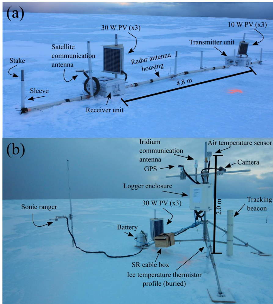
Figure 2: Instruments installed on Petermann Ice Island-A-1-f on 20 October 2015. (a) Stationary ice penetrating radar (sIPR) components deployed with antennas ‘in-line’ and attached to eight sleeves that slid over stake anchors. (b) Automatic weather station components, including a camera that acquired a weekly image of the sIPR and ablation stakes (not shown). The two systems were installed 30 m apart on two small ridges at the location denoted in Fig. 1c. PV = photovoltaic panel, SR = sonic ranger.
