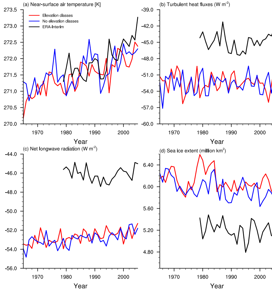
Figure S1. Annual means of selected climate variables in the simulations EC-1K (“No elevation classes”, blue) and EC-6K (“elevation classes”, red), and ERA-Interim (only 1979-2005, black) for reference. The data are area-weighted averages (integrated for sea-ice) for the region in Fig. 5.
