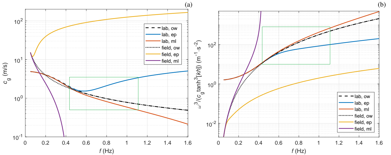
Figure 1. Group velocity c_g (a) and the ratio \omega^3/(c_g \tanh^3[kh]) (b) versus wave frequency f = \omega/(2\pi) , computed for thin laboratory ice (test series 3000 from the LS-WICE experiment analyzed in Part B) and for field conditions with h = 1000 m, \rho_w = 1025 kg/m 3 , \rho_i = 910 kg/m 3 , E = 6 \cdot 10^9 Pa, h_i = 1.5 m. The corresponding open water solutions are shown in black (note that the two black curves overlap for f > 0.5 Hz). Green rectangles mark regions covered by the LS-WICE experiment.
