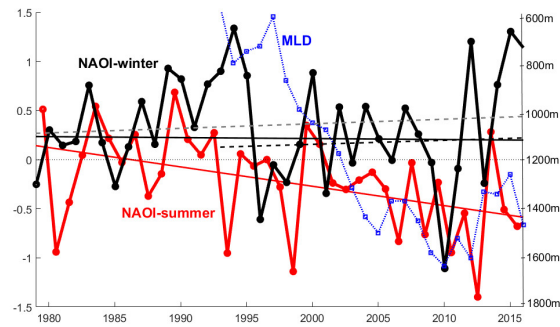
Figure 7. Cold season NAO index (black, November-April) and warm season NAO index (red, May-October) with linear trends. Additionally plotted are the trends of cold season NAO index since 1993 (black dashed line, October-April) and for winter season (gray dashed line, January-April). The blue line shows maximum MLD in the Greenland Sea derived from ARMOR data-set (see Bashmachnikov et al. (2019) for details).
