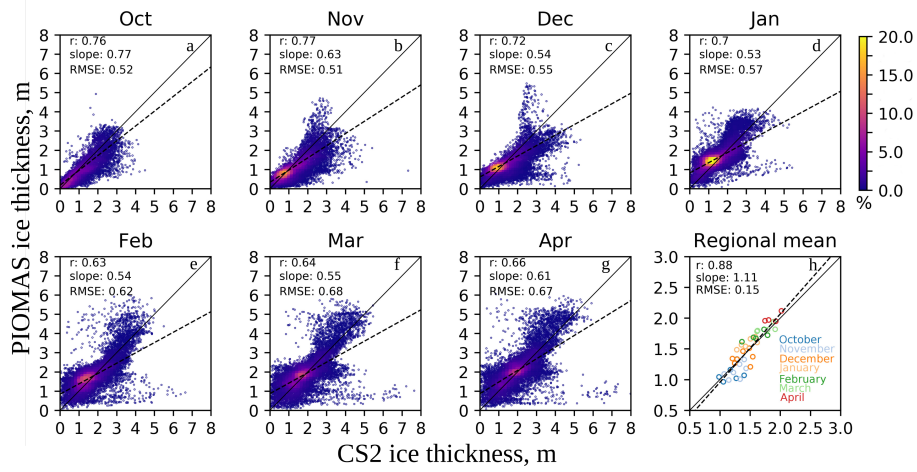
Figure 2. Density scatter plots of PIOMAS and CS2 monthly effective sea ice thickness (m) in the Greenland Sea, October-April 2010-2016: (a-g) - each point corresponds to one grid-cell sea ice thickness; (h) mean monthly sea ice thickness over the ice covered area of the Greenland Sea for all inter-compared snapshots. The color of the points in panel h corresponds to a month. The dashed lines show the linear regression fit and the solid lines are 45° angles. The correlation coefficients (r), the slope of the linear regressions and the root-mean-square error (RMSE) are given in the upper left corner.
