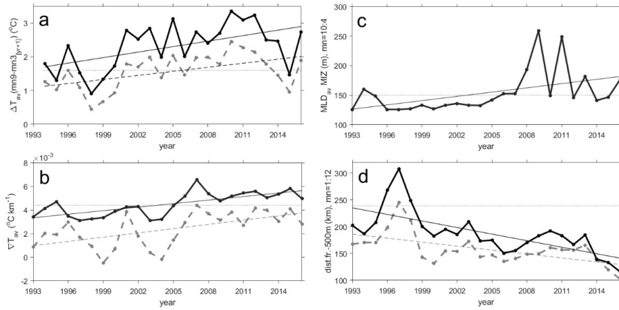
Figure 6. Interannual variations of water properties, averaged over the MIZ area. (a) Temperature drop ( ^{\circ}\text{C} ) from maximum in September to minimum in April next year; (b) annual mean temperature gradient across the MIZ ( ^{\circ}\text{C km}^{-1} ); (c) the mixed layer depth (m), averaged over the cold season; (d) annual mean distance of the 3^{\circ}\text{C} isotherm from the shelf break (km). In panels (a), (b) and (d) solid black line – data averaged over the upper 50-m layer, dashed gray line – over the upper 200-m layer. In panel (d) 3^{\circ}\text{C} isotherm is shown for the 50-m means and 2^{\circ}\text{C} – for the 200-m means.
