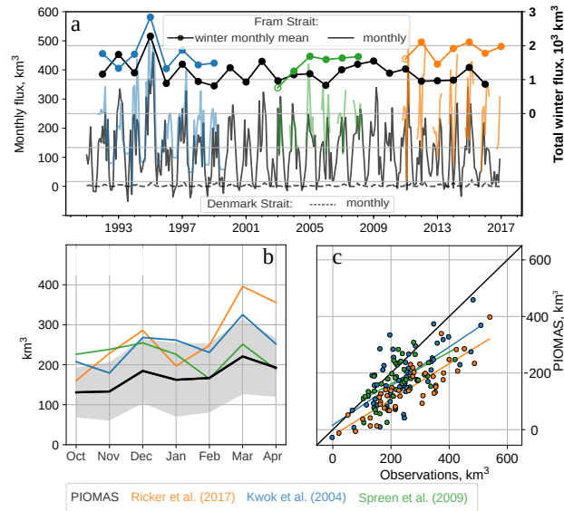
Figure 3. Sea ice volume fluxes ( \text{km}^3 ): a - time series of PIOMAS and observation-based monthly sea ice volume fluxes through Fram and the Denmark Straits, 1991-2016 (note that the total winter fluxes are referenced to the right scale). Empty circles indicate seasons with an incomplete winter cycle; b - winter intra-annual cycle sea ice volume flux through Fram Strait, averaged over the period of the observations and over 1991-2016 for PIOMAS data-set. The gray background color correspond to one standard deviation interval from the PIOMAS mean; c - scatter diagram of monthly mean PIOMAS sea ice volume fluxes through Fram Strait versus monthly mean observations.
