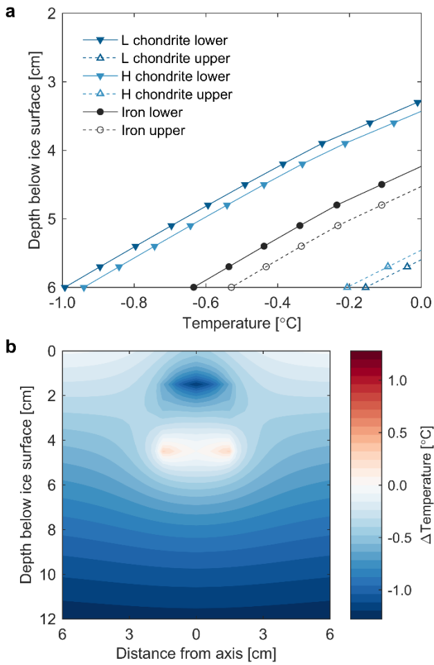
Figure 10. (a) Maximum temperatures reached at the upper and lower surfaces of L chondrites, H chondrites and iron meteorites when their positions are fixed. Depths are with reference to their centres. In all cases meteorites are 3 cm in height and 3 cm in width. (b) Cross-section of difference in temperature fields surrounding an iron meteorite vs an L chondrite when the basal temperature in each case first reaches 0 °C.
