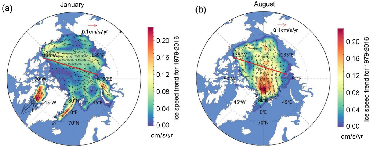
5 Figure 5. Sea ice motion trend in (a) January and (b) August. The magnitude of ice motion is indicated by background color and the length of arrows.
