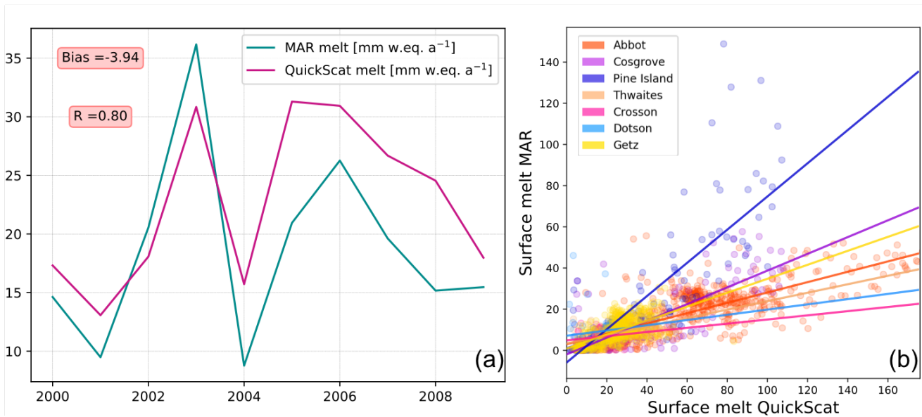
340 Figure 6 : (a) Time series of surface melt rates in mean over the model domain derived from satellite data and simulated by MAR, years labelled on the X-axis refer to the second year of a given austral summer (e.g., summer 1999–2000 is labelled 2000). and (b) Surface melt modelled versus surface melt interpolated from satellite data (QuickScat) over drainage basins, (only where surface melt > 0 mm w.e. a -1 ) and over the period 1999-2009.
