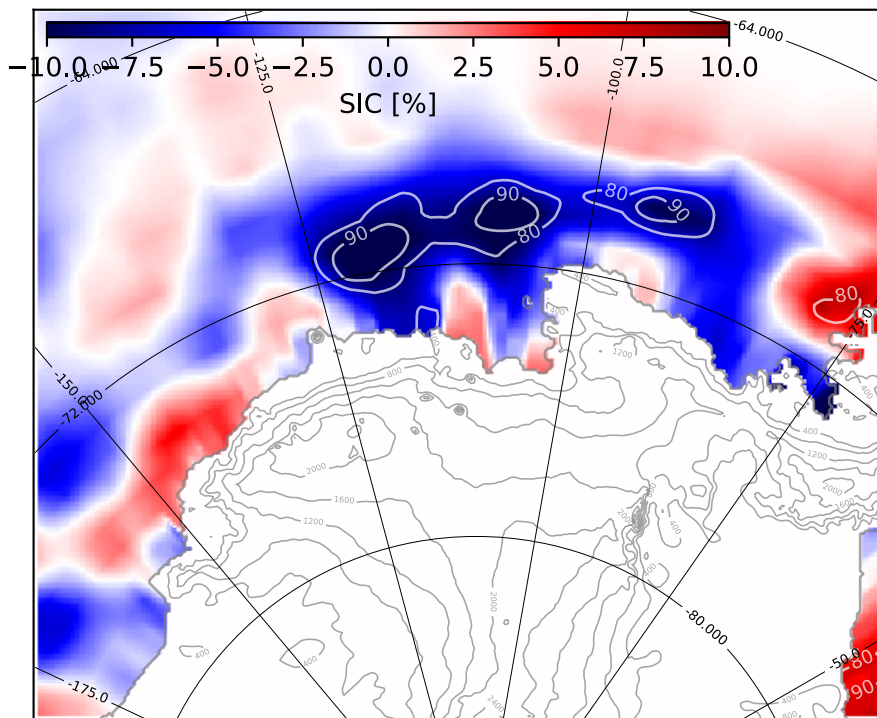
Figure 14 : Summer sea ice cover (%) anomaly (composites minus the climatology over 1979-2017) during El Niño events in JJA (6 month before). Contours represent significance with Welch's t-test.
