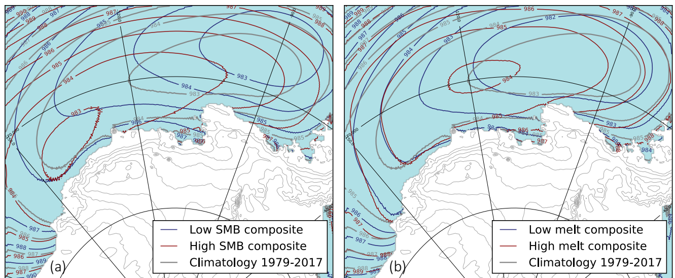
395 Figure 8 : Summer sea surface pressure composites for high/low SMB (a) and high/low surface melt (b). The ice-sheet height is indicated by thin grey contours (every 500m).
