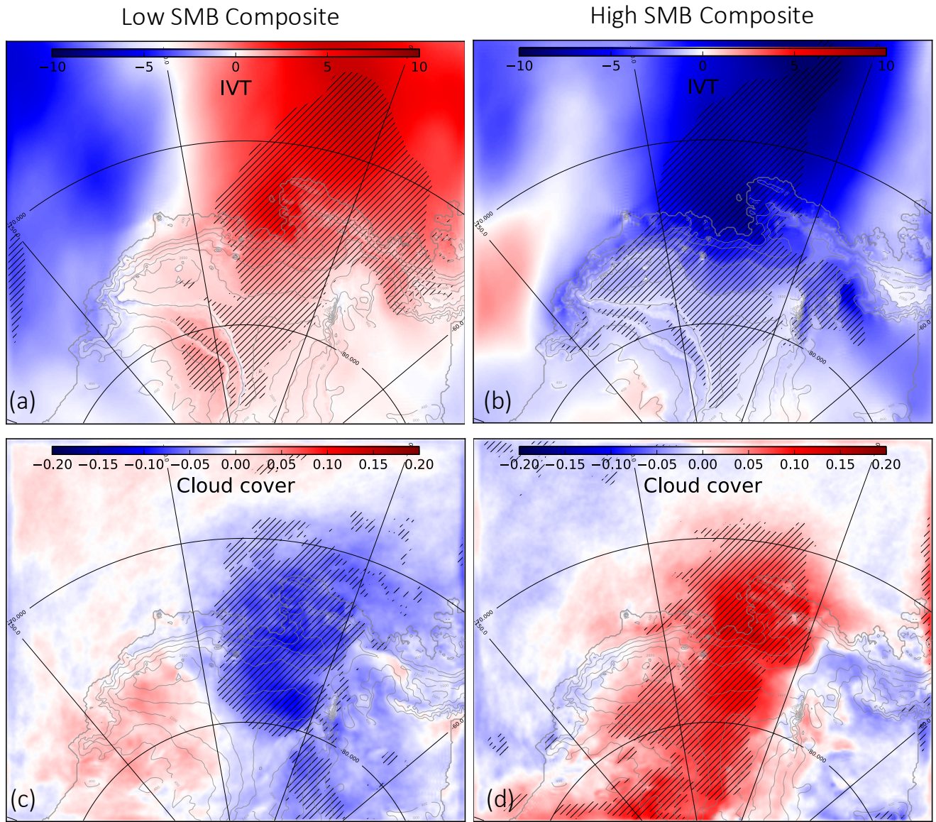
Figure 10 : (a,b) vertical Integrated Vapor Transport (IVT) along the y-axis (negative toward the continent) calculated as IVT [kg m^{-2}] = \int_{925}^{700} q \cdot v \frac{dP}{g} , with q the specific humidity ( g kg^{-1} ), v the wind speed ( m s^{-1} ), P the pressure (Pa), and g the gravity ( 9.81 m s^{-2} ) and (c,d) cloud cover (no units, from 0 to 1) anomalies during low-SMB summers (left) and high-SMB summers (right). Anomalies are calculated as high/low composites minus the climatology over 1979-2017. Hatched area represents significance >90% calculated with Welch's t -test.
