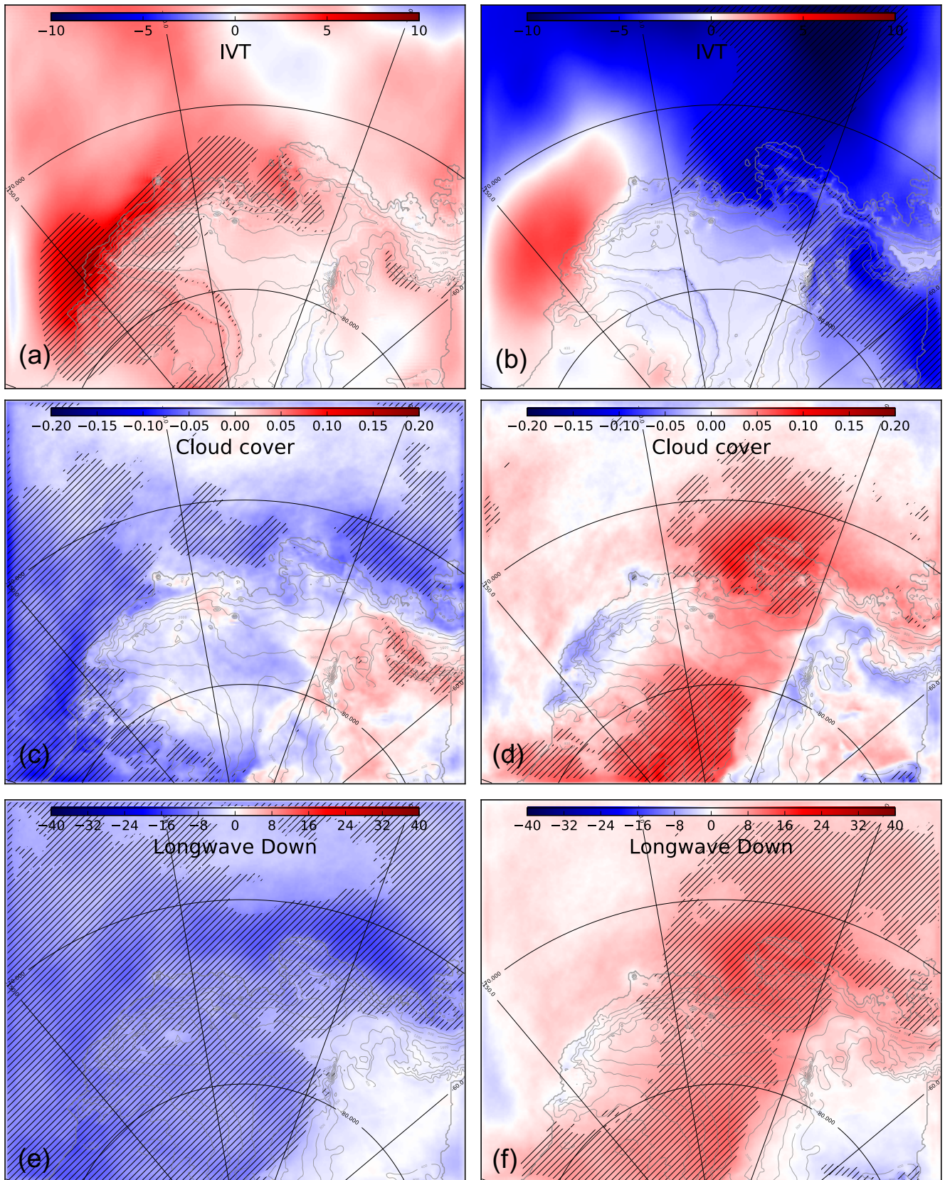
Figure 11 : (a,b) vertical Integrated Vapor Transport (IVT) along y axis (negative toward the continent ( \text{kg m}^{-2} ) (same formula as for Fig.10), (c,d) cloud cover (no units, from 0 to 1), and (e,f) downward longwave radiation ( \text{W m}^{-2} ) anomalies during low-melt summers (left) and high-melt summers (right). Anomalies are calculated as high/low composites minus the climatology over 1979-2017. Hatched area represents significance >90% calculated with Welch's t -test.
