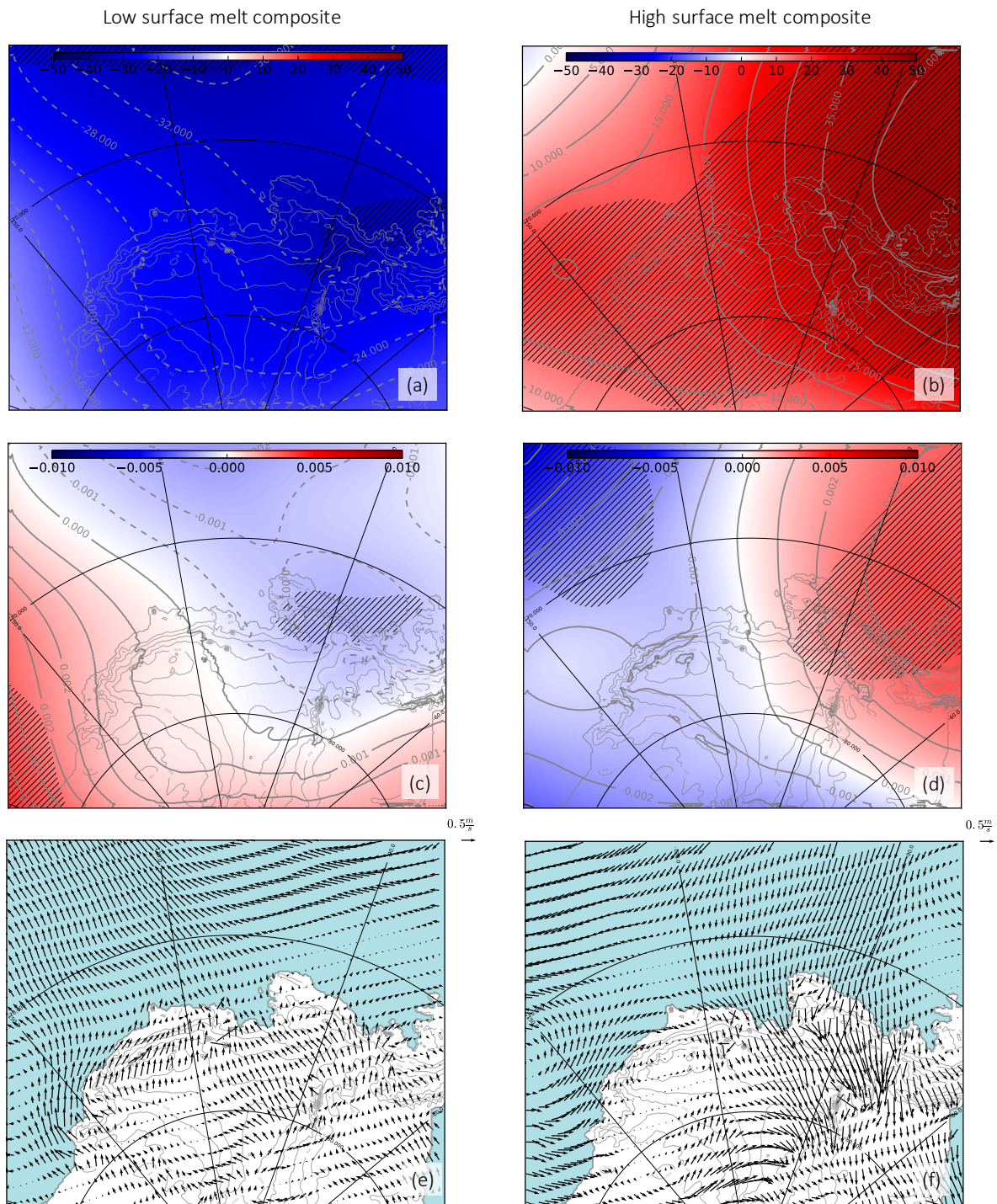
465 Figure 12 : (a,b) 500 hPa geopotential height (m) and (c,d) 500 hPa geopotential height divided by the domain-averaged value for each season and (e,f) 10m wind ( \text{m s}^{-1} ) anomalies during low-melt summers (left) and high-melt summers (right), scales of arrow lengths are shown near the upper right corner of panels (e) and (f). Anomalies are calculated as high/low composites minus the climatology over 1979-2017. Hatched area represents significance >90% calculated with Welch's t -test.
