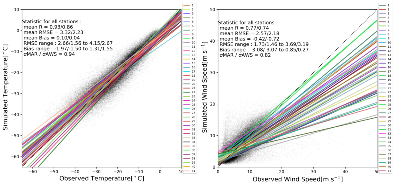
Figure 2 : Scatter plots of observed vs. simulated daily near-surface temperature (a) and daily near-surface wind speed (b) for the selected AWS (see corresponding locations and names in Fig. 1). The statistics, including RMSE, correlation (R), bias, and standard deviations ( \sigma ), are calculated for individual stations and provided as multi-station mean over the whole year / over the summer months (DJF). The range of RMSE and biases across individual stations is also indicated with the 10 th percentile and the 90 th percentile of all RMSE values. The lines represent least-mean-square linear fit between simulated data and observations. The complete statistical analyses for individual AWS are provided in Supplementary material (Table S1-S2).
