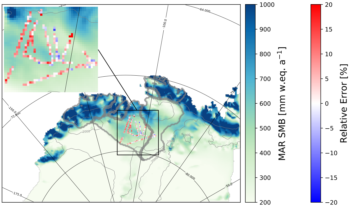
Figure 3 : Annual mean (1979-2017) simulated SMB (blue-green scale) and relative error of the simulated SMB compared to the airborne-radar data from Medley et al. (2013, 2014) (blue-red color bar). Grey contours indicate the surface height (every 1000m). The drainage basins under consideration are the same as in Fig.1 (large grey contours here).
