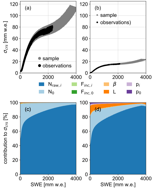
Figure 3. Precision of SWE calculated by means of error propagation. (a) and (b) show the absolute precision with grey dots as a synthetic data set and black dots as the in situ observations. (c) and (d) show the relative contribution of each parameter to the overall precision. (a) and (c) present the results based on hourly observations while (b) and (d) show the results of the daily observations.
