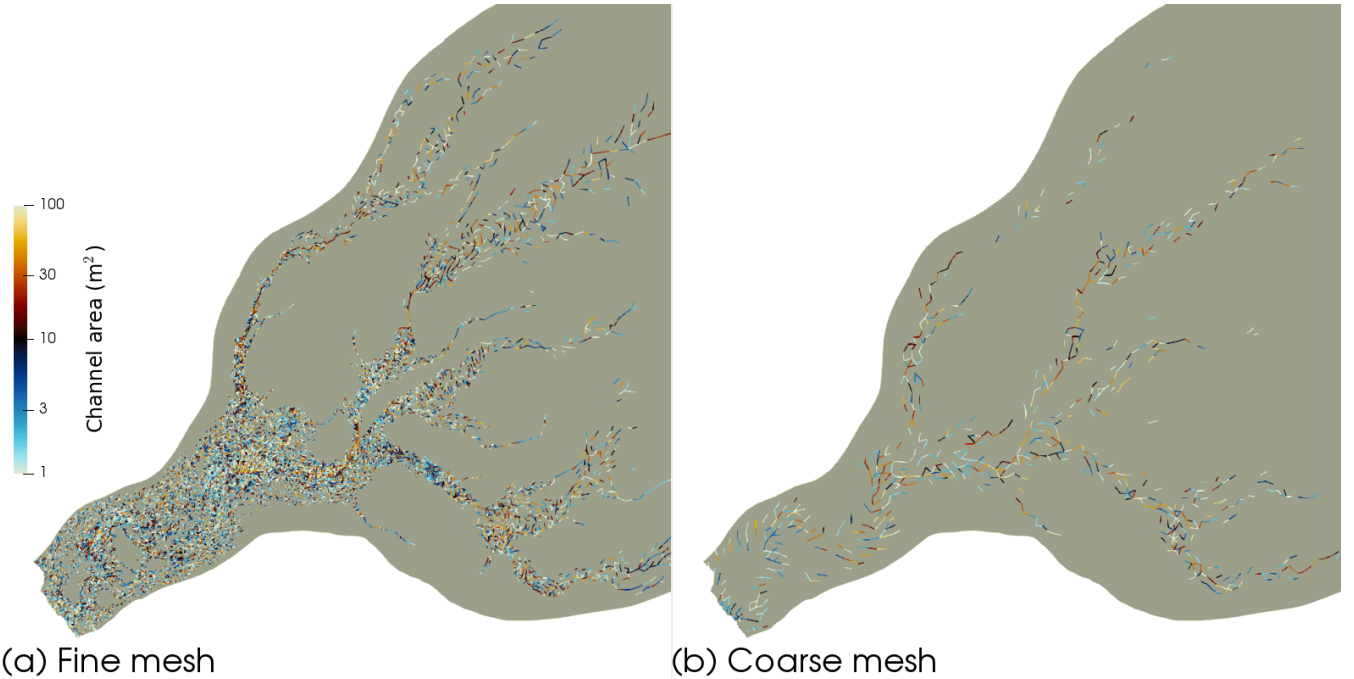
Fig. 13 – Comparison of hydrological model results for different mesh resolutions. (a) The standard, fine mesh described in Sect. 2.3.; (b) a coarser, 500 m-resolution mesh. Note that the overall layout of the channel network is virtually identical between the two.
