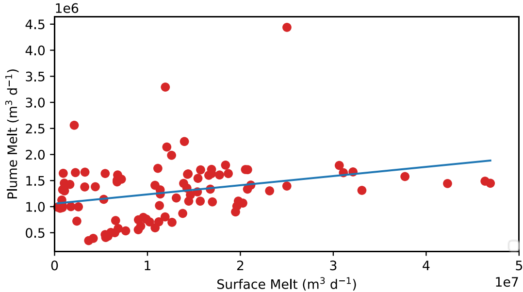
Fig. 11 – Scatter plot of surface melt versus plume melt for SummerDaily17 run, showing low correlation. The line of best fit is shown in blue.
