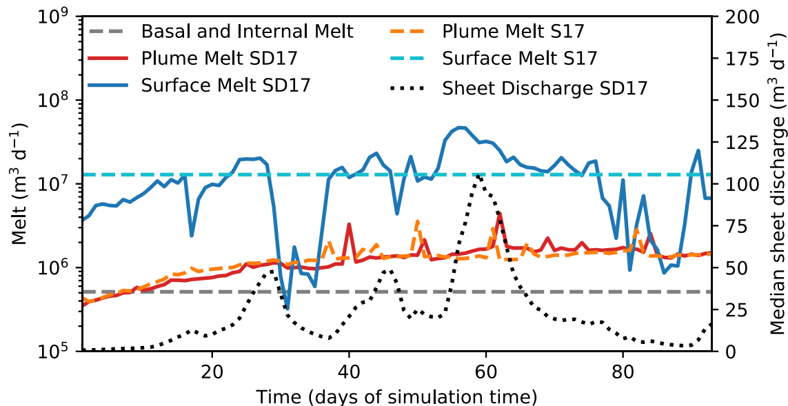
Fig. 8 – Time series of melt sources in SummerDaily17 (red and blue solid lines) and SummerAverage17 (orange and light blue dashed lines) model runs. Note logarithmic y-axis. Basal and internal melt was constant across both runs and is included for comparative purposes – note how plume melt is of equal or greater importance. Median sheet discharge (dotted line; taken as the median over the whole model domain) shows response of subglacial hydrological system to surface melt, and evolution of the system towards greater channelisation over melt season.
