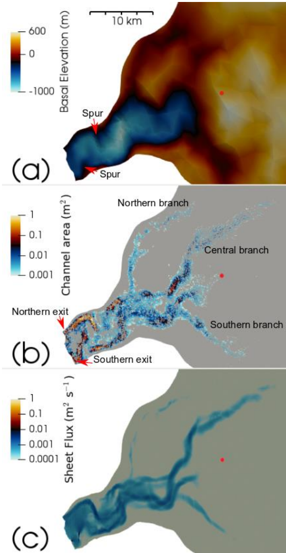
Fig. 3 – Winter hydrological system at Store at end of Winter run and basal topography. (a) bed elevation; (b) channel area ; (c) sheet flux. The red dot in all panels marks the location of the S30 site from Young et al. (2019). Channels and sheet drainage pathways can be seen to largely follow the deeper parts of the bed. We have shown very small channels and low sheet discharges to fully display the existence of a connected winter drainage system.
