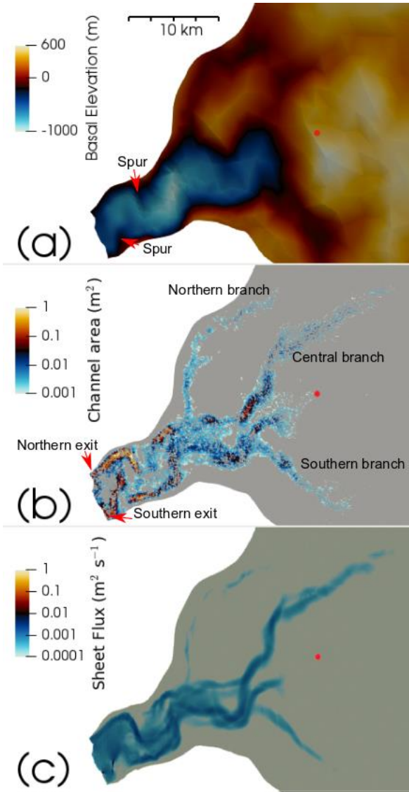
Fig. 3 – Winter hydrological system at Store at end of Winter run and basal topography. (a) bed elevation; (b) channel area ; (c) sheet flux. The red dot in all panels (a) and (b) marks the location of the S30 site from Young et al. (2019). Channels and sheet drainage pathways can be seen to largely follow the deeper parts of the bed. We have shown very small channels and low sheet discharges to fully display the existence of a connected winter drainage system.
