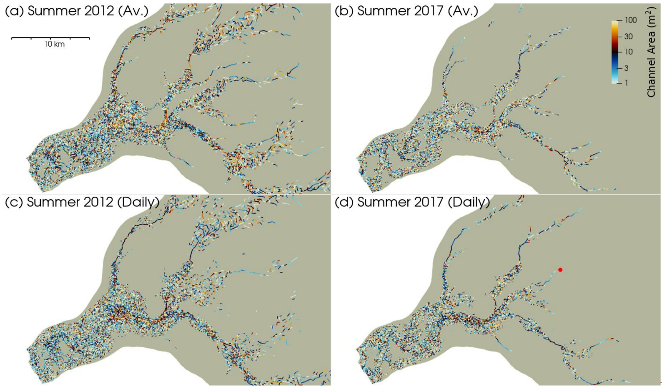
Fig. 5 – Summer channel network of Store. (a) SummerAverage12 model run; (b) SummerAverage17; (c) SummerDaily12; (d) SummerDaily17 (red dot shows S30 study site from Young et al. (2019)). All the panels show the channel network at the end of the respective simulations, after three months of surface melting. The daily-forced runs show a less extensive channel network owing to declining surface melt towards the end of the melt season.
