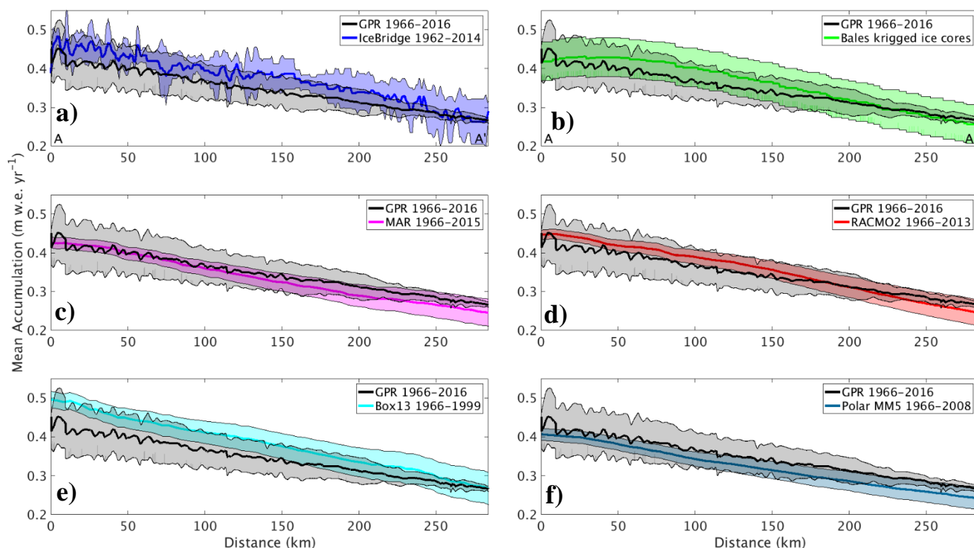
456 Figure 7. Average GreenTrACS GPR accumulation rates (black) compared with a) IceBridge accumulation radar, b) Bales09 krigged 457 ice core map, c) MAR, d) RACMO2, e) Box13, and f) Polar MM5. GPR measurements are statistically indistinguishable from each of 458 the other measurements along this 285 km transect in the dry snow zone (A – A' on Figure 1). 459
