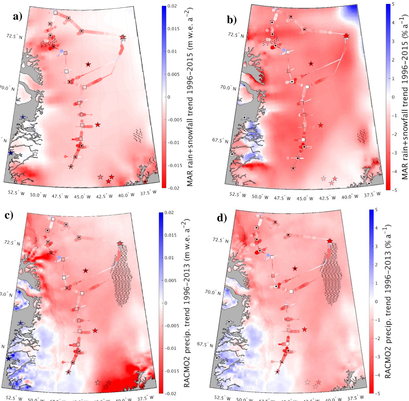
Figure 10. Best fit linear trends for each grid cell showing magnitude (left) and percent (right) changes in total precipitation for a) and b) MAR (1996 – 2015) and c) and d) RACMO2 (1996 – 2013). Statistically significant RCM grid cell trends are stippled black. Also shown are accumulation trends for GreenTrACS firn cores (squares), ACT10A, ACT10B, ACT10C, D4, D5, Katie, Sandy, Summit 2010, and Raven/Dye-2 cores (stars on ice sheet) and precipitation trends from Mernild et al (2014; stars on coast) with statistically significant trends indicated by black dots.
