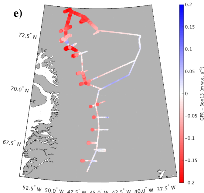
Figure 9. Differences between GreenTrACS accumulation rates and a) Polar MM5, b) MAR, c) Bales09, d) RACMO2, and e) Box13 accumulation rates averaged over the corresponding time periods. Large dots show statistically significant differences from GreenTrACS accumulation rates.
