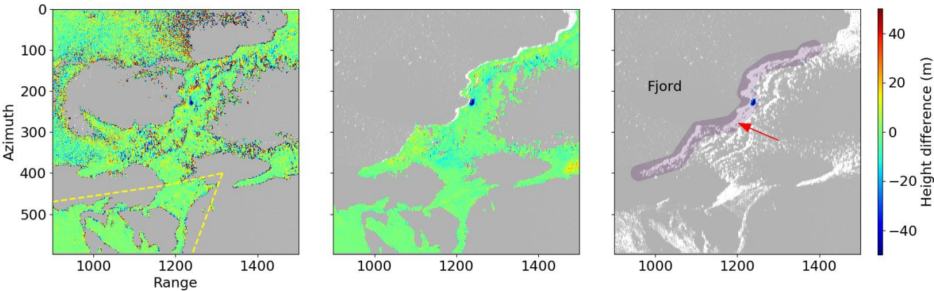
Figure 4: Example of a calving event extraction on 20 August 16:40 UTC in radar geometry. The left image shows the elevation difference between two unstacked DEMs, while in the middle the difference is calculated between two stacked DEMs. The right
