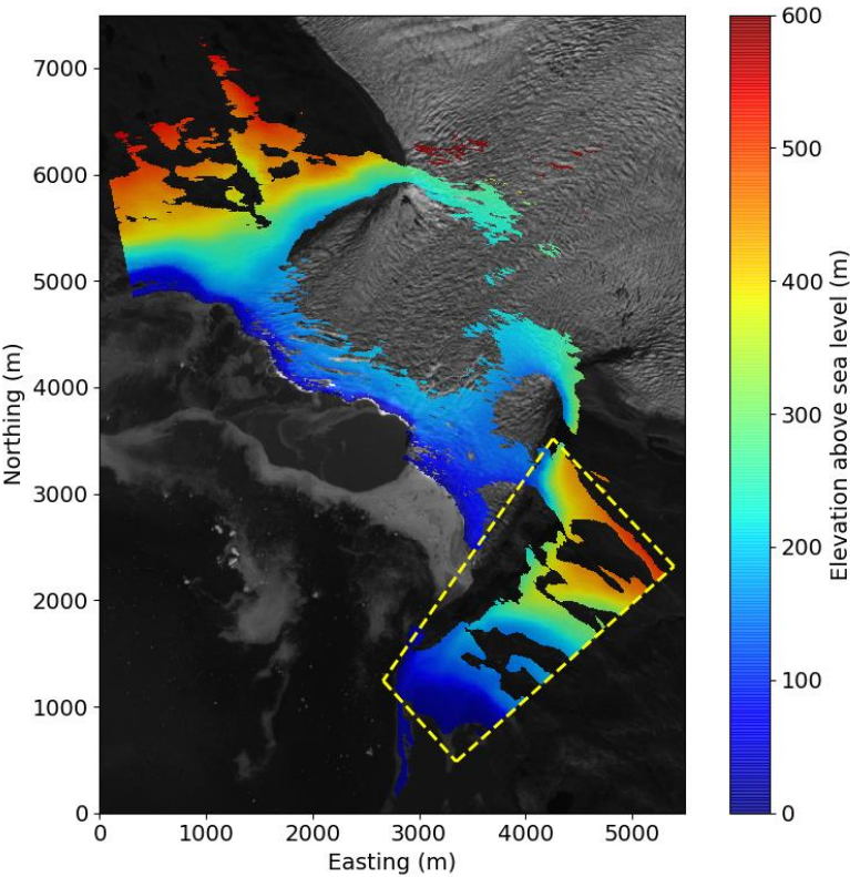
Figure 33: TRI derived DEM stacked over 60 minutes. The yellow square marks the stable terrain area where the mean variability was investigated. The origin of the coordinate system corresponds to 527350 E / 7739550 N (UTM 22N). Background: Sentinel-2A scene from 3 August 2016 (from ESA Copernicus Science Hub: https://scihub.copernicus.eu ).
