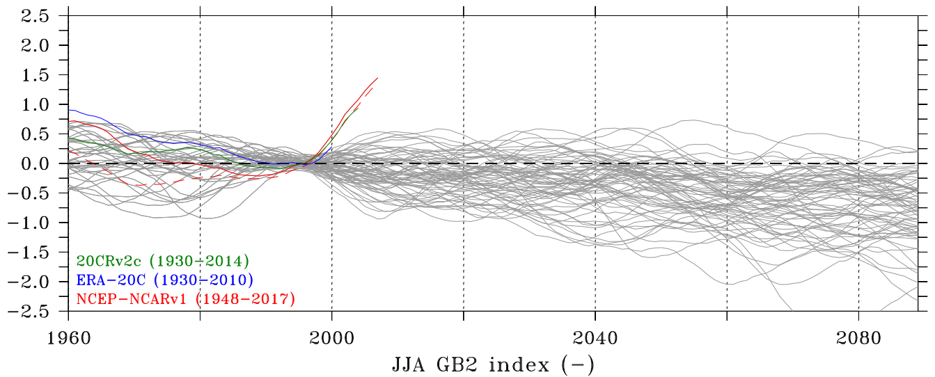
Figure 1. Time series of JJA GB1 (dashed red line) and GB2 index (solid red line) indices over 1950-2100 as simulated by NCEP/NCAR v1 reanalysis (red line), by 20CRv2c reanalysis (green line), by ERA-20C ERA-20C reanalysis in blue as well as simulated by all the CMIP5 models (grey lines) for which both RCP4.5 and RCP8.5 scenarios are available. For the CMIP5-based time series, the Historical scenario is used over 1900-2005 and both RCP4.5 and RCP8.5 afterwards. A 20-year running mean has been applied to smooth the time series, and values have been normalised (average = 0 and standard deviation = 1) using 1986-2005 as reference period. The NCEP-NCARv1-based GB1 index is also shown (dashed red line).
