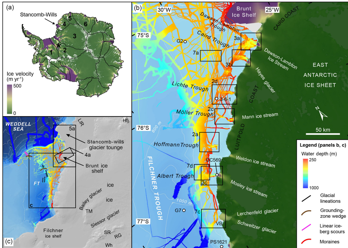
Figure 1. Location maps of the Coats Land margin, East Antarctica. (a) Map of Antarctica with ICESat-derived drainage basins ( http://icesat4.gsfc.nasa.gov/cryo_data/ant_grn_drainage_systems.php ) and MEaSUREs ice velocities (Rignot et al., 2011). The study area is the south-western part of Antarctic Drainage System 4. To the south of the study area, Antarctic Drainage System 3 discharges into the Thiel Trough and Filchner Ice Shelf via the Bailey Ice Stream, Slessor, Recovery and Support Force glaciers. To the north Antarctic Drainage Systems 5 and 6 discharge into the ice shelves of Dronning Maud Land. The black star is the Pensacola Mountains. (b) The continental shelf and glaciology of the eastern Weddell Sea showing the multibeam-bathymetry coverage (for survey details see text); regional bathymetry is from IBCSO v. 1.0; Arndt et al. (2013). Hfj. is Heimefrontfjella; TM is Theron Mountains; SR is Shackleton Range; RG is Recovery Glacier; Wh is Whichaway Nunataks; LIR is Lyddan Ice Rise. Also shown is the location of offshore glacial landforms described in Larter et al. (2012) and Arndt et al. (2017). Labelled boxes show the locations of Figs. 1c, 4a and 5a. (c) Detailed map showing multibeam-bathymetry coverage in glacial troughs of the Coats Land margin and eastern Weddell Sea and the MEaSUREs ice velocities of regional glaciers and ice streams. The location of datasets shown in Figs. 2, 3 and 7 is marked by labelled boxes. Labelled white circles with a black borders show the locations of sediment coring sites. VB is Vahsel Bay.
