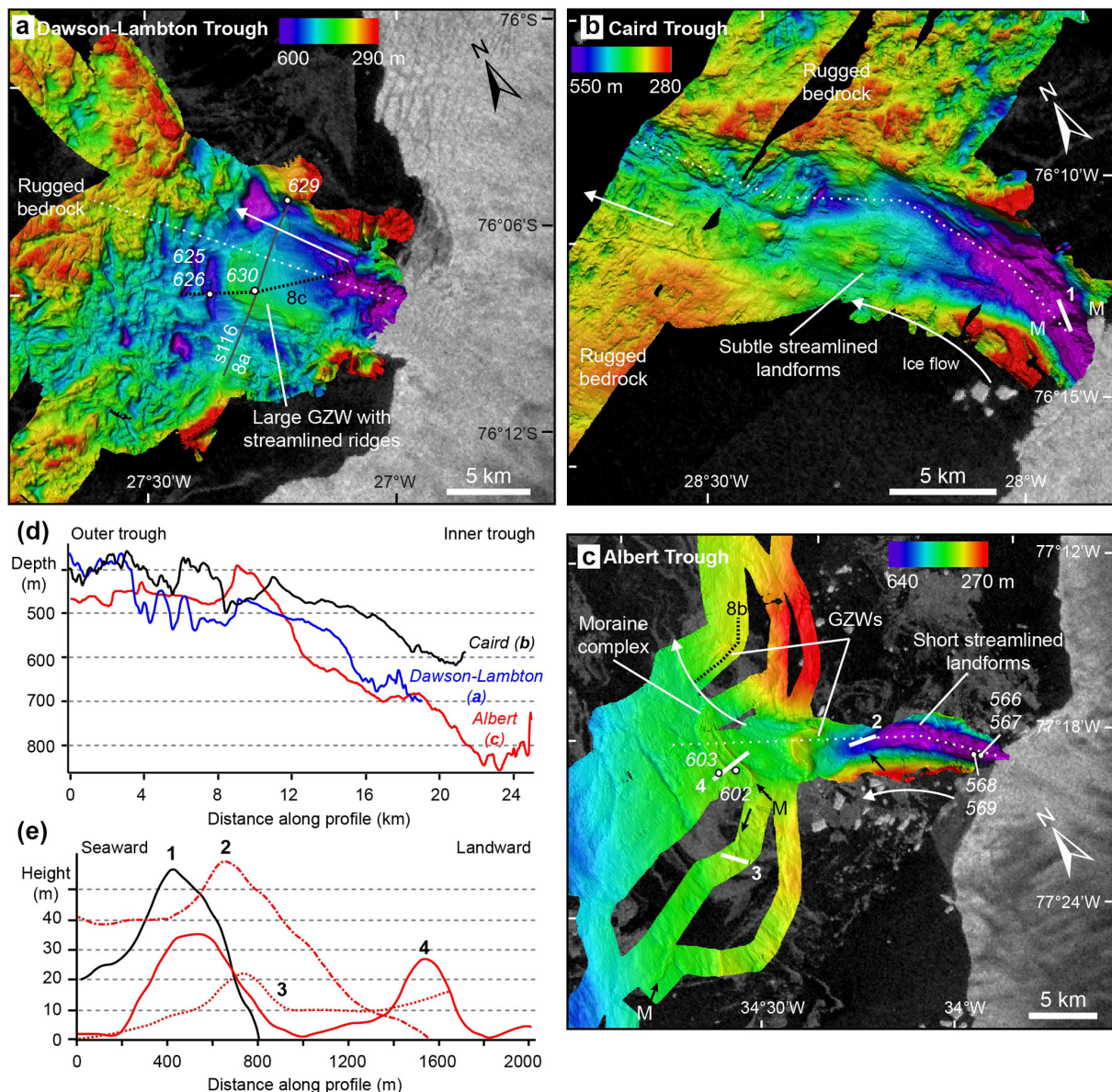
Figure 3. Geomorphology of glacial troughs downstream of high-velocity glaciers ( 250\text{--}500\text{ myr}^{-1} ). Black line shows the location of seismic-reflection profile BAS101-s116 along the strike of the large grounding-zone wedge (GZW) in (a) Dawson-Lambton Trough, (b) Caird Trough and (c) Albert Trough, with labelled examples of streamlined landforms, moraines (arrowed and labelled “M”) and GZWs. (d) Long profiles down the central axis of the troughs showing landward-dipping geometries; profile locations are marked with white dotted lines in panels (a), (b) and (c). (e) Cross profiles over prominent ridge features interpreted as moraines; profile locations are marked with solid white lines in panels (b) and (c). Sediment core locations are marked by white circles with associated core numbers.
