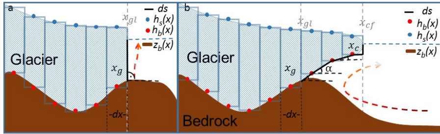
Figure 1. Visualization of the 1D glacier model with the staggered grid for a) a tidewater glacier and b) a glacier with a floating tongue. Red dots indicate where the depth of glacier base h_b is defined and blue dots where surface elevation h_s of the glacier is defined. They are calculated at dx/2 - the half width of each grid cell. Last grounded cell has the coordinate x_g and last floating cell has the coordinate x_c . The grounding line x_{gl} is determined at the border of the last grounded cell, where the flotation criterion is not yet achieved. After the grounding line, the calculation of submarine melt along the distance ds (thick, black line) is performed with the line plume model. For a floating tongue (b) every grid cell may have a different angle for the slope of glacial base while for a tidewater glacier (a) the angle is set to 90 degrees. The bedrock elevation z_b (brown, thick line) is equal to h_b for the grounded part and is deeper for the floating part of the glacier.
