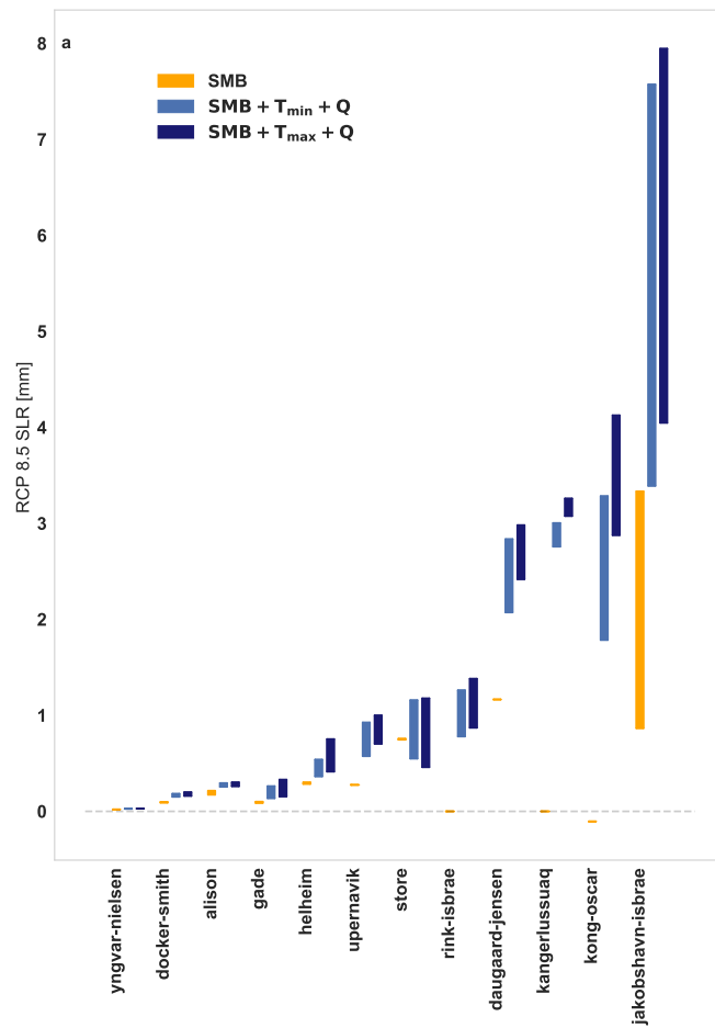
Figure 12. First to third quartile of contribution to SLR for each glacier. Future RCP 8.5 scenarios were either forced with SMB changes only (orange) or changes in SMB, ocean temperature ( T_{\min} and T_{\max} ) and subglacial discharge (blue).
