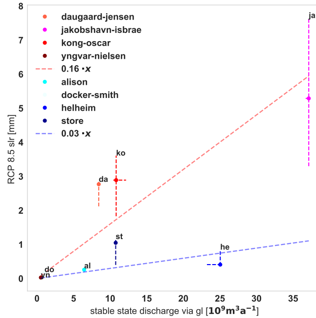
Figure 13. First to third quartile (median indicated with a dot) of contribution to SLR under RCP 8.5 for 8 glaciers from Table 3 as a function of the present-day grounding line discharge. The future simulations were forced by changes in SMB, subglacial discharge and minimal and maximal ocean temperature trend (Tab. 1). Dashed lines indicate a linear function of the present-day grounding line discharge in future SLR for 2100 obtained with an ordinary least square model from the median values for 4 glaciers only that result in a high slope (reddish colors) and that result in a low slope (blueish colors). For the reddish glaciers, the resulting slope and p-value are 0.03 \text{ mm km}^{-3} \text{ a} and 0.18 respectively, and for the blueish glaciers 0.16 \text{ mm km}^{-3} \text{ a} and 0.01.
