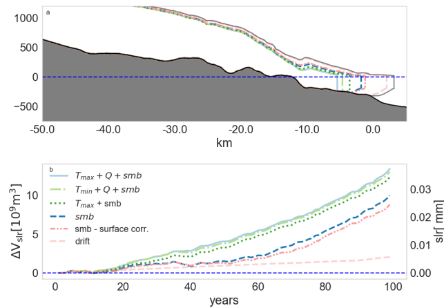
Figure 10. a) Yngvar Nielsen Glacier with a representative medium-slretreat scenario applying forcing factors as subglacial discharge Q , ocean temperature T , surface mass balance \text{smb} with and without accounting for surface elevation correction ( \text{smb} - \text{surface corr.} ) for the medium SLR scenario. The corresponding SLR of each experiment is displayed in panel b).
