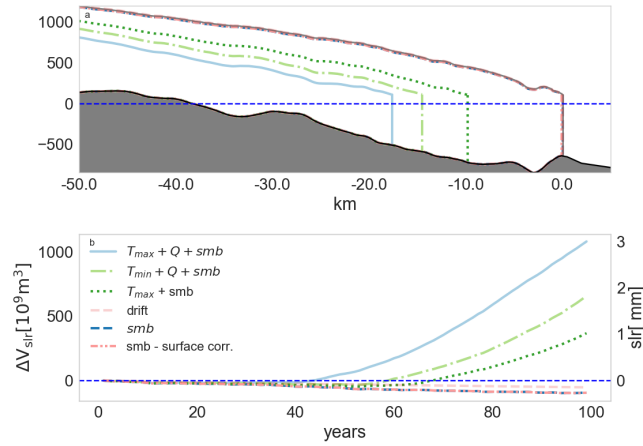
Figure 9. a) Kong-Oscar Glacier with a representative medium-slretreat scenario applying forcing factors as subglacial discharge Q , ocean temperature T , surface mass balance \text{smb} with and without accounting for surface elevation correction ( \text{smb} - \text{surface corr.} ) for the medium SLR scenario. The corresponding SLR of each experiment is displayed in panel b).
