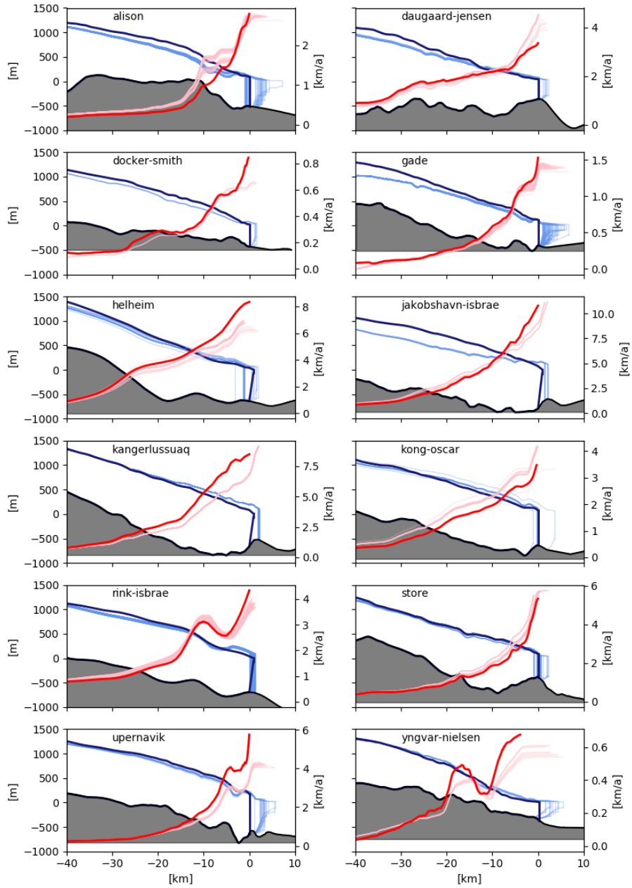
Figure 6. Simulated glacier elevation (light blue) and velocity profile (light red) for the last 40 km to the grounding line depicted together with observational data (dark blue and dark red) by Morlighem et al. (2014) and Rignot and Mouginot (2012). Bedrock data is derived by the flux weighted average over the whole catchment area. The number of simulations is given in Tab. S3, supporting information
