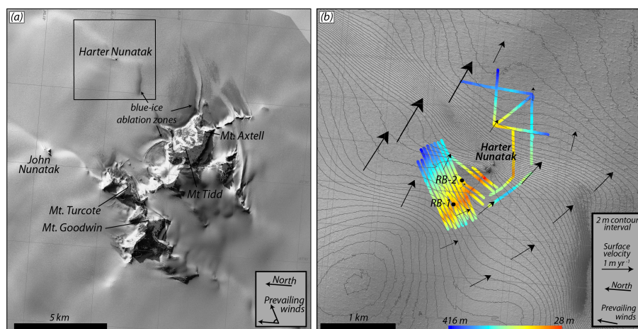
Figure 4. (a) WorldView satellite imagery (copyright DigitalGlobe, Inc.) of the Pirrit Hills. Black box shows the location of panel (b). (b) Map of Harter Nunatak (center) and the surrounding area. Elevation contours are derived from WorldView satellite imagery (DEM created by the Polar Geospatial Center). Colors represent ice thickness as measured with radar surveys. Arrows represent ice velocity and were measured by repeat stake surveys. The ice velocity measured closest to the RB-2 drill site is \sim 0.25 m yr^{-1} . Changes in ice-surface elevation were also measured at these stakes.
