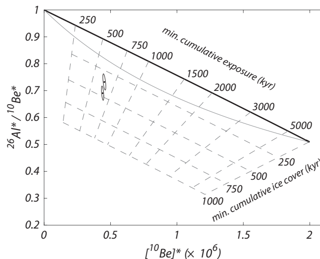
Figure 6. ^{10}\text{Be} and ^{26}\text{Al} data for the bedrock samples from Harter Nunatak shown in Fig. 5c. Nuclide concentrations are normalized to the surface production rate for each sample ( N^* = N/P , where N is the ^{10}\text{Be} or ^{26}\text{Al} concentration and P is the local production rate of that nuclide). Ellipses represent 1\sigma uncertainty regions. Continuously exposed and uneroded surfaces will plot along the black line near the top. Continuously exposed and eroding surfaces will plot between the black line and the solid gray line. Samples plotting below the solid gray line, such as those from Harter Nunatak, require at least one episode of ice cover following prior exposure. Dashed contours show lower limits on the cumulative exposure and cumulative ice cover experienced by the samples.
