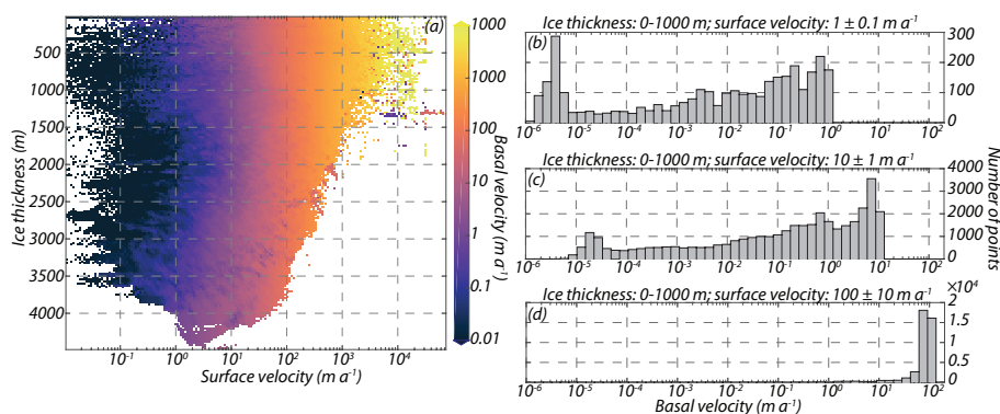
Figure 3. (a) The relationship between surface velocity, ice thickness, and basal velocity, as predicted by the 5 Myr ice-sheet model. Results for the full ice sheet are binned by surface velocity and ice thickness, and each bin is colored by its average basal velocity. This averaging hides considerable variability in the actual range of basal velocities within each bin. Therefore, in panels (b-d), we provide histograms of basal velocity for points in the model where the ice is less than 1000 m thick, for surface velocities of \sim 1 , \sim 10 , and \sim 100 m/yr. At depths relevant to subglacial drilling, significant subglacial erosion is unlikely in areas where the surface velocity is less than \sim 10 m/yr (see Fig. 1).
