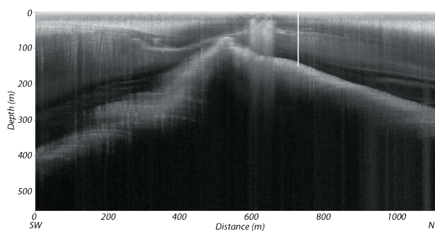
Figure 7. Unmigrated radar profile collected with the CReSIS accumulation radar showing the location of the 150 m RB-2 borehole to the bed. Profile is oriented perpendicular to the ridge.
