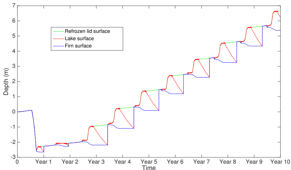
Figure 2. The development of surface melt lakes over a 10 year model run using 2010-11 data. Here, the blue line shows the firm surface, the red line the lake surface, and the green the refrozen lid. On the vertical axis 0 is the initial ice shelf surface.
