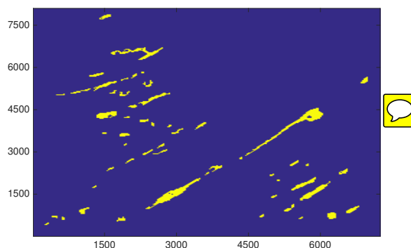
Figure 4. Landsat image of a section of the Larsen C Ice Shelf where melt lakes were present on 06/01/2016. Both axes have units of meters. Here the lakes are coloured yellow and areas where lakes were not present are coloured blue. Although this data was taken from the Landsat 8 mission so is from a later time than the lakes examined using the 2010-11 melt season, it is likely that the lakes will be similar in many aspects due to the role of topography in the location of lake basins.
