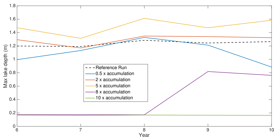
Figure 6. The maximum lake depth for years 6-10 of the simulations carried out for varying snow depths.
