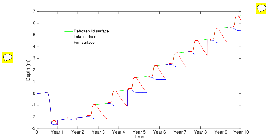
Figure 2. The development of surface melt lakes over a 10 year model run using 2010-11 data. Here, the blue line shows the firm surface, the red line the lake surface, and the green the refrozen lid. On the vertical axis 0 is the initial ice shelf surface.
