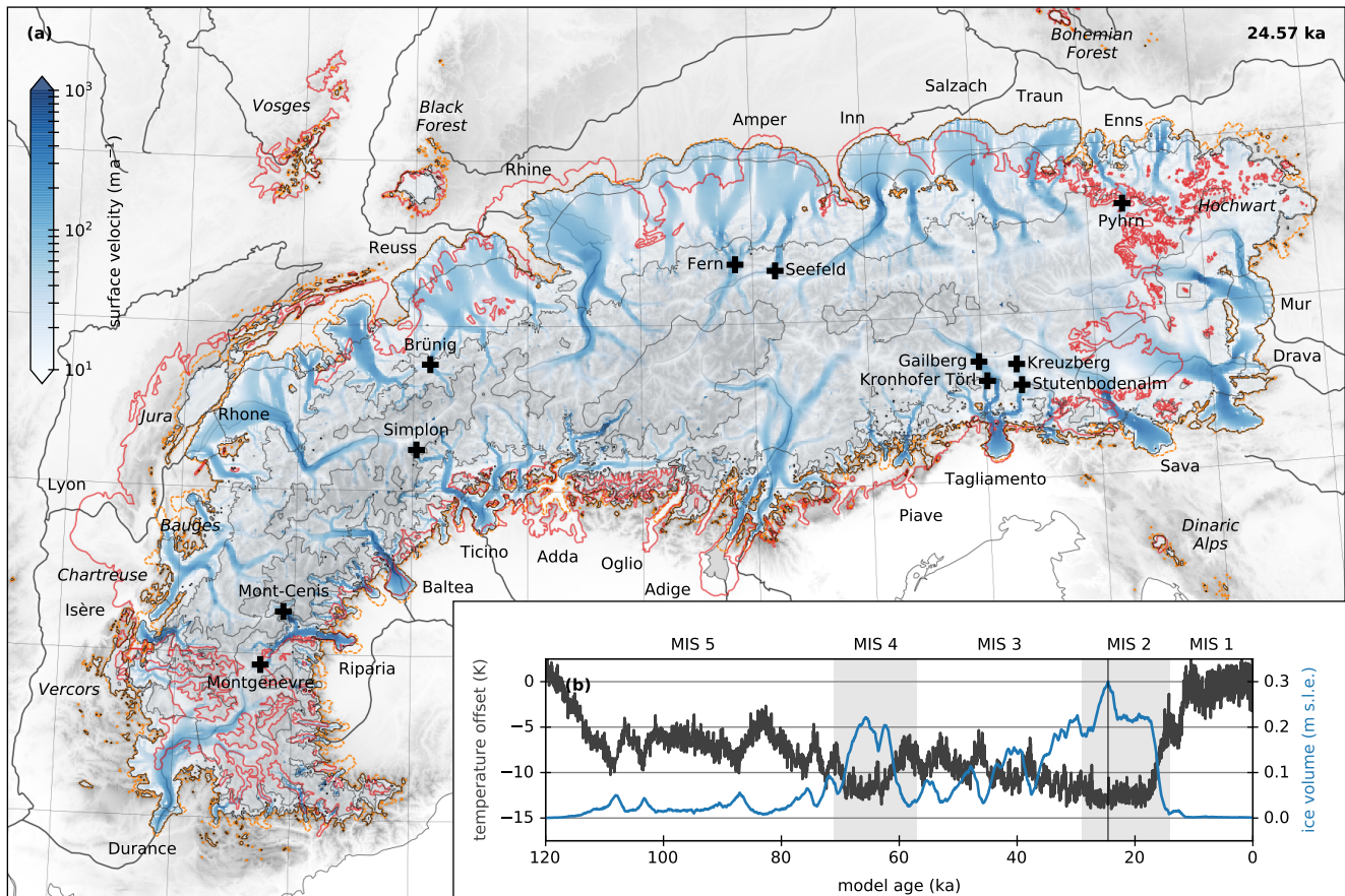
Figure 4. (a) Modelled bedrock topography (grey), ice surface topography (200 m contours), and ice surface velocity (blue) in the Alps 24.57 ka before present, corresponding to the maximum modelled ice cover. The modelled LGM ice extent (dashed orange line) and geomorphological reconstruction (solid red line, Ehlers et al., 2011), and some major transfluences across mountain passes (crosses) are shown. (b) Temperature offset time-series from the EPICA ice core used as palaeo-climate forcing for the ice flow model (black curve, Jouzel et al., 2007), and modelled total ice volume through the last glacial cycle (120–0 ka), expressed in meters of sea level equivalent (m s.l.e., blue curve). Shaded gray areas indicate the timing for Marine Oxygen Isotope Stage (MIS) 2 and MIS 4 according to a global compilation of benthic \delta^{18}O records (Lisiecki and Raymo, 2005).
