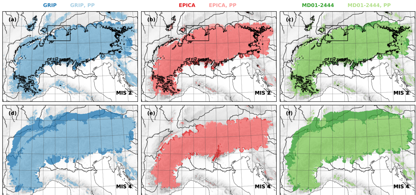
Figure 3. (a–c) Cumulative extent of modelled ice cover extent during MIS 2 (29–14 ka), without (dark colours) and with (light colours) palaeo-precipitation corrections, and using temperature time-series scaling factors (Table 2) adjusted to model the area glaciated by the Rhine glacier piedmont lobe (black rectangle) in agreement with the Last Glacial Maximum (LGM) geomorphological reconstruction (solid red line, Ehlers et al., 2011) (solid black line, Ehlers et al., 2011). (d–f) Cumulative extent of modelled ice cover extent during MIS 4 (71–57 ka). Only the simulation driven by the EPICA temperature time-series yields reasonable realistic MIS 4 ice cover.
