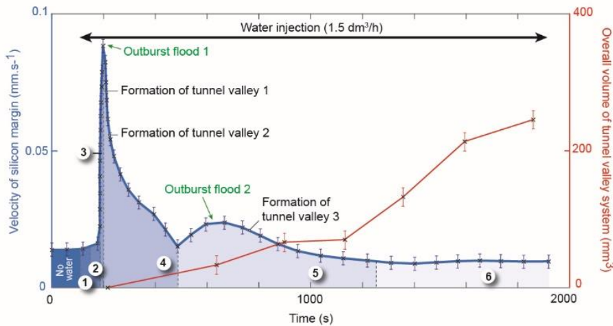
373 374 Figure 5. Progressive expansion of overall volume of tunnel valleys system vs. velocity of silicon 375 margin through the experiment. The circled numbers correspond to the six-stages of the proposed ice 376 stream lifecycle.
