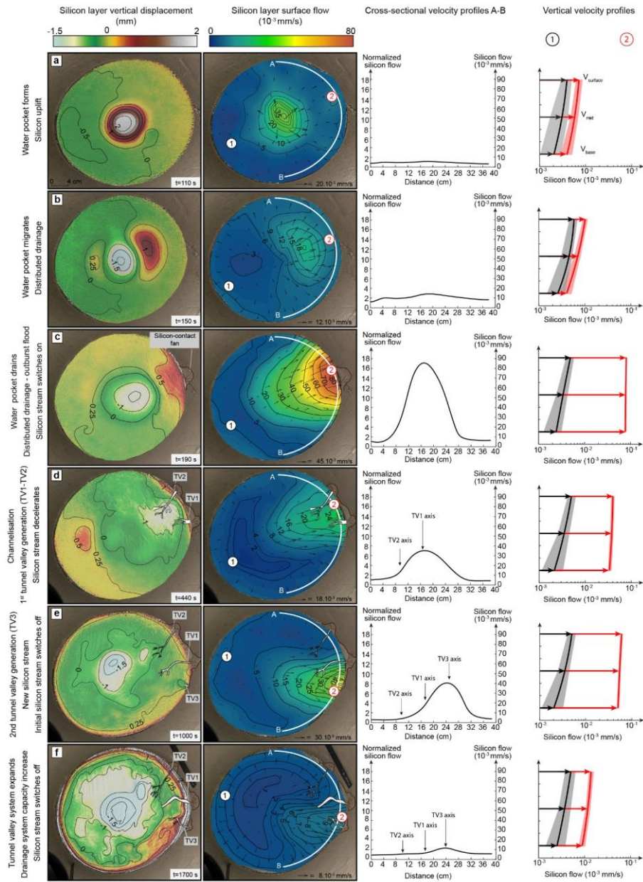
284 285 Figure 3. Temporal evolution of the experiment. a, Formation of water pocket, uplift of silicon surface 286 uplift and acceleration. b, Migration of water pocket and overlying region of uplift and accelerated flow. 287 c, Marginal drainage of water pocket and onset of silicon streaming. d, Tunnel valley development and 288 silicon stream deceleration. e, Formation, migration and marginal drainage of a new water pocket,
