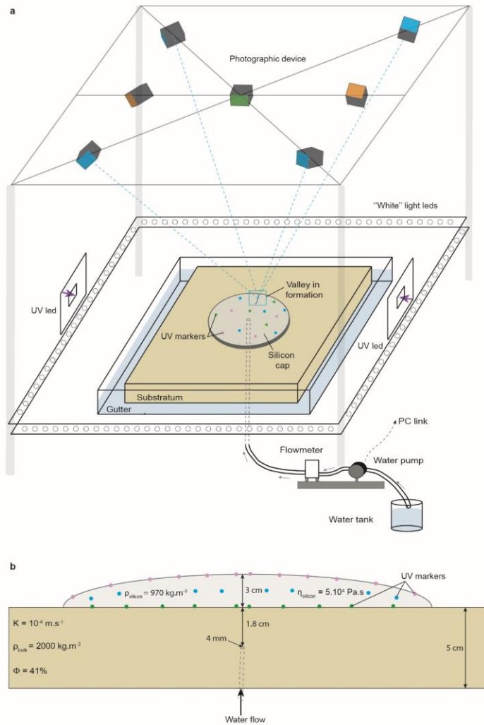
229 Figure 1. Description of the analogue device used in this study. a, Overview of the analogue device. 230 The analogue device consists in a 70 cm long, 70 cm wide and 5 cm deep glass box filled with saturated 231 and compacted sand simulating the substratum. The ice sheet portion is simulated by a circular layer of 232 silicon putty containing 3 levels of UV markers. Meltwater production is simulated by a central and 233 punctual injection of pure water within the substratum. Five synchronized cameras placed above the 234 silicon putty (in blue) focus on the tunnel valley system and are used to produce digital elevation models 235 by photogrammetry. Another camera (in orange) takes overview photographs of the analogue device to 236 follow the progress of the whole experiment. A last camera (in green) is positioned at the vertical of the 237 silicon layer centre and is configured to take high-resolution photographs in black light of the UV 238 markers (illuminated with two lateral UV led lights). b, Cross-sectional profile of the analogue device 239 displaying the position of the UV markers and the physical characteristics of both the substratum and 240 the silicon layer.
