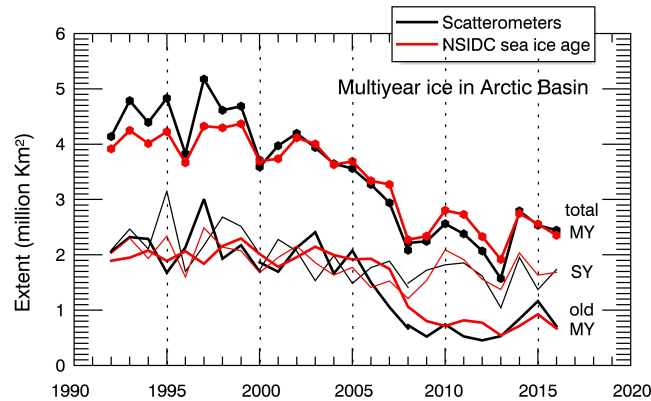
5 Figure 12: Time series of monthly wintertime (March) total multiyear sea ice extents (segmented into SY and older MY classes) within the Arctic Basin from the scattermeter (black) and the NSIDC sea ice age (red) records.
