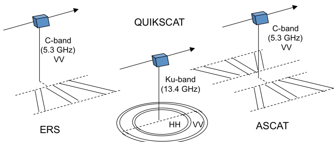
Figure 2: Observation geometries of the satellite scatterometers.
