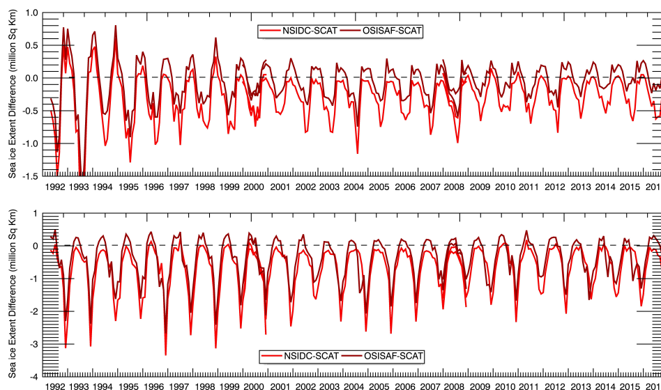
Figure 5: Time series of scatterometer sea ice extent differences to passive microwave (SSMI-based) products from NSIDC-0051 and OSISAF-409a from 1992 to 2016 for the Arctic (top) and Antarctic (bottom).
