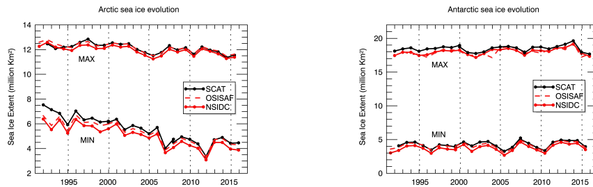
Figure 8: Evolution of minimum and maximum monthly sea ice extents from scatterometers (black line) and passive microwaves (continuous and dashed red lines) from 1992 to 2016 for the Arctic (left) and Antarctic (right).
