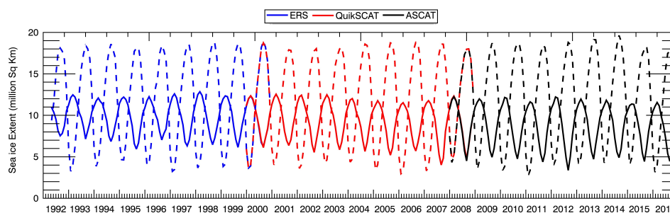
Figure 4: Time series of monthly Arctic (continuous) and Antarctic (dashed) scatterometer sea ice extents from 1992 to 2016.
