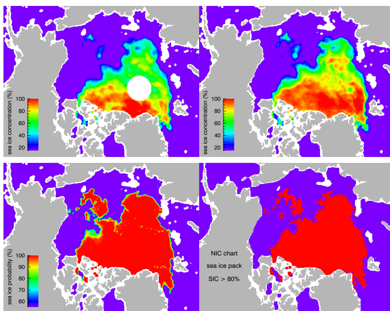
10 Figure 7: Comparison of summer sea ice extents on September 15 th 2016 from passive microwaves (NSIDC-0051 top left, OSISAF-450 top right), active microwaves (ASCAT, bottom left) and NIC sea ice charts (bottom right). The color scales represent sea ice concentration (top panels), sea ice probability (bottom left panel) and NIC sea ice concentration larger than 80%.
