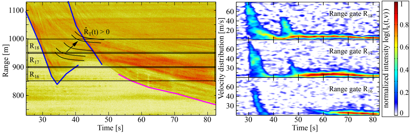
Figure 4. Detail of complete transition from bottom panels of Fig. 2. Left: MTI with location of Doppler range gates. The location of transition R_T is not fixed, but moves upward with time \dot{R}_T(t) > 0 . Right panels: Doppler velocity distribution in range gates R_{16} (850–900 m), R_{17} (900–950 m) and R_{18} (950–1000 m).
