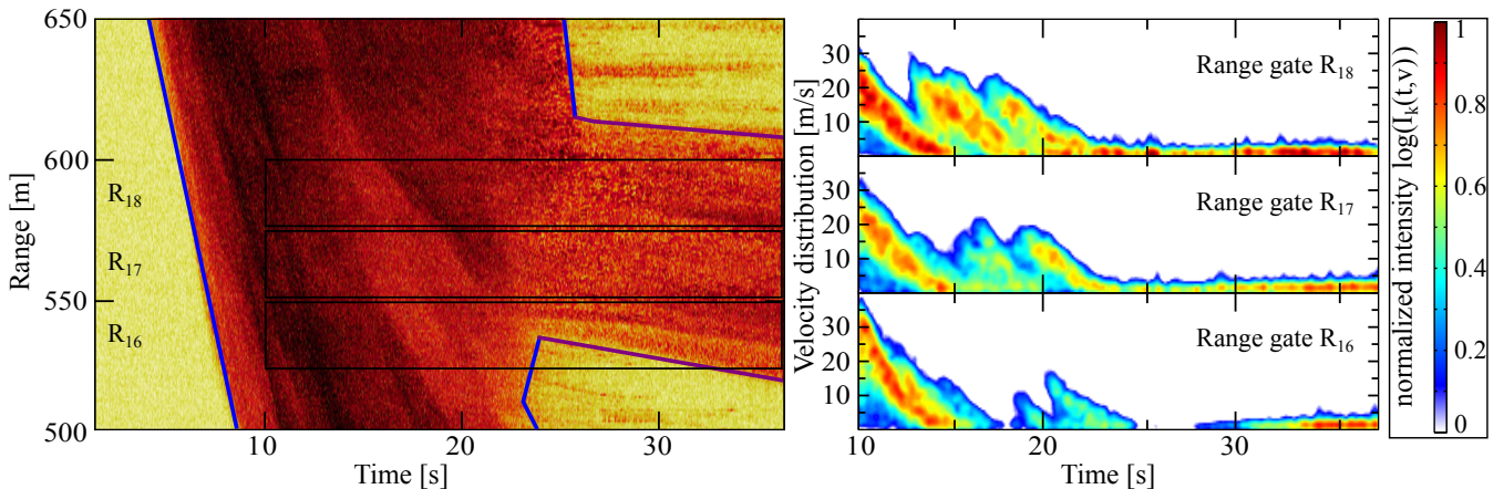
Figure 3. Detail of a partial transition from avalanche #17-3030 from the top panels of Fig. 2. Left: Zoomed MTI plot with location of Doppler range gates. Right panels: Doppler velocity distribution in the ranges gates R_{16} (525–550 m), R_{17} (550–575 m) and R_{18} (575–600 m).
