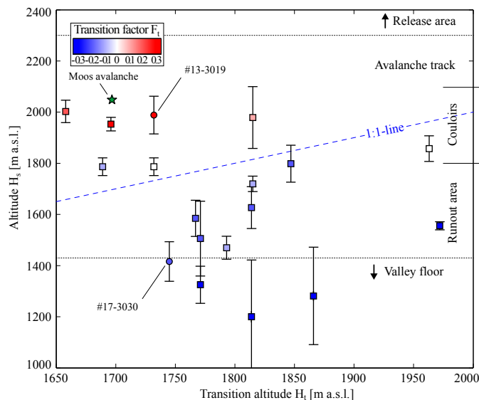
Figure 6. Altitude of transition, H_t , against the altitude of the -1\text{ }^\circ\text{C} line, H_s . The 1:1-line (dashed blue) divides the avalanches into cases where the transition occurs above or below the H_s -line. Horizontal dashed lines and annotation on the right side characterize roughly the VdIS terrain. The colour indicate the transition index from Figure 5.
