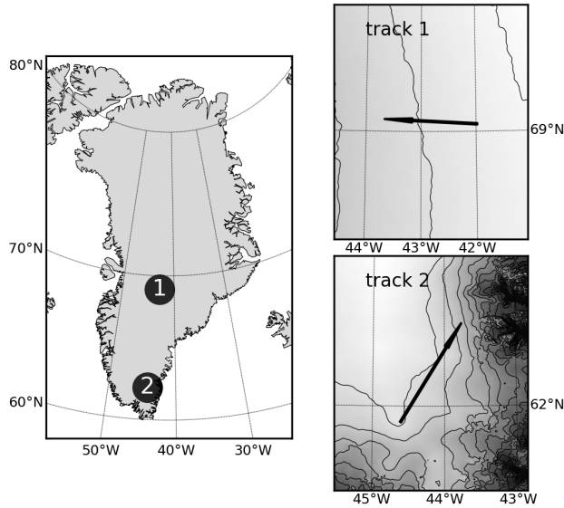
Figure 2. MCRDS surveys on a map. The map of Greenland is plotted using a stereographic projection with a central meridian of 41^\circ W and a central parallel of 72^\circ N. Isolines on maps correspond to a surface elevation change of 250 m.
