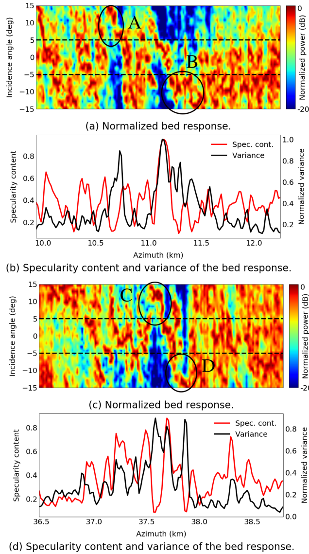
Figure 11. Specularity content and variance as measures of specularity of the bed return for track 2. For comparison we take two parts of track 2 each 2.3km long. The power of the angular energy returns (a) and (c) is normalized with respect to the highest value of the distribution at each azimuth position. The area inside the dashed horizontal lines in (a) and (c) corresponds to \Delta\theta_1 .
