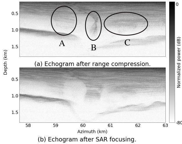
Figure 14. Stretching and shrinkage of internal layers in range-compressed data of track 2. The range compressed echogram is at the top, the SAR focused echogram is at the bottom.
