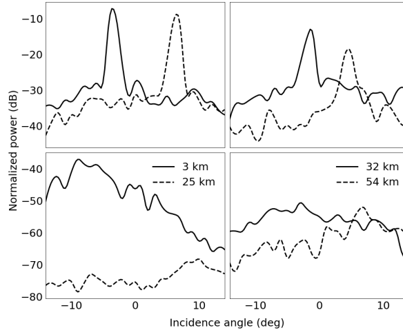
Figure 6. Internal layer (top panel) and bed (bottom panel) returns for track 2 at azimuth positions x = (3, 25, 32, 54) km, marked with vertical red lines in Fig. 4(a). Quadratic interpolation was applied to smooth the signatures.
