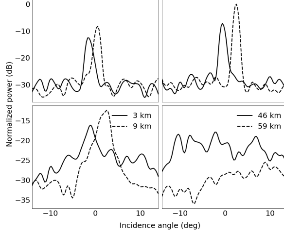
Figure 5. Internal layer (top panel) and bed (bottom panel) returns for track 1 at azimuth positions x = (3, 9, 46, 59) km, marked with vertical red lines in Fig. 3(a). Quadratic interpolation was applied to smooth the signatures.
