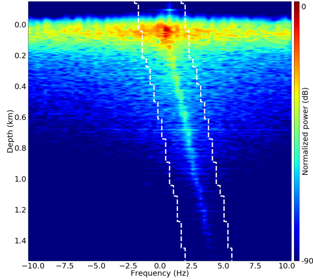
Figure 7. Azimuth spectrum of a 250m-long SAR block in track 1, azimuth position x = 59 km. The frequency interval \hat{f}_{\text{layer}}(d) \pm 0.05\Delta B_{\text{az}} is marked with white lines.
