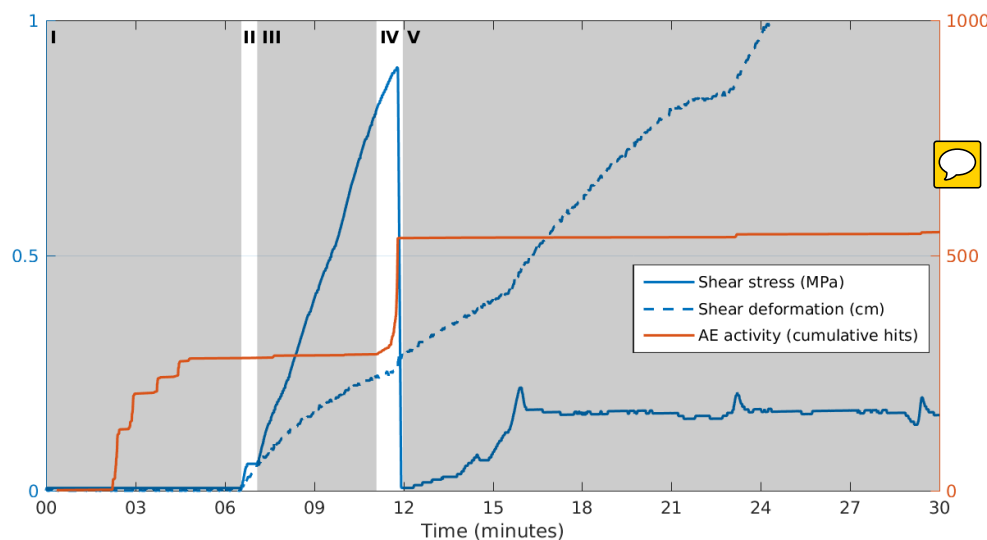
Figure 4: Typical curves of shear stress at failure, shear deformation and acoustic activity for a shear test at T = -3\text{ °C} and \sigma = 200\text{ kPa} . I-V represent the typical stages of each experiment: Consolidation (I), sample fitting to shear rings (II), pre-peak shear deformation (III), shear failure (IV) and post-peak shear strength. Rupture is clearly detectable by the strong decrease in shear stress. An increase in the evolution of the cumulative AE hits can be observed before rupture.
