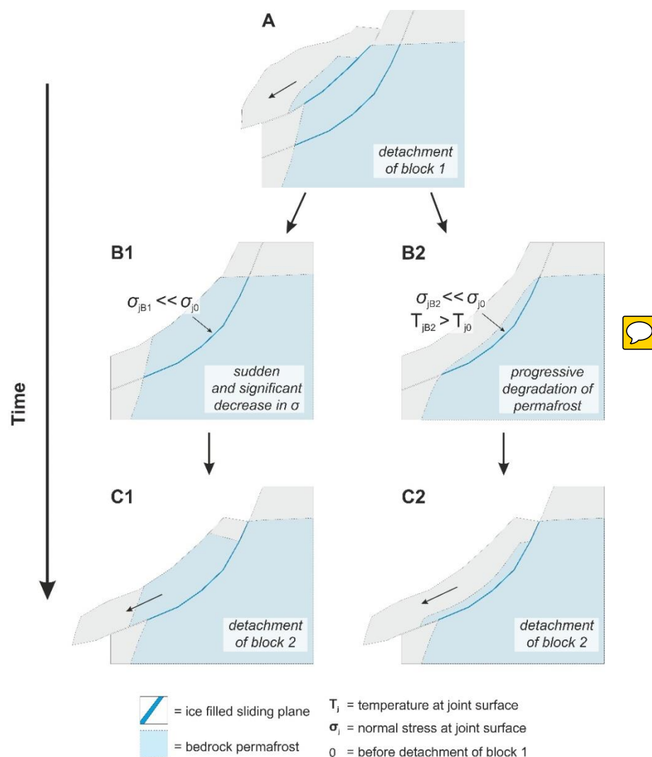
495 Figure 10: Progressive failure in a warming permafrost rock slope displaying thermal and normal stress conditions before and after detachment of a first slab. Both (B2) progressive thermal warming (i.e. permafrost degradation), but even faster (B1) sudden unloading can initiate failure.
