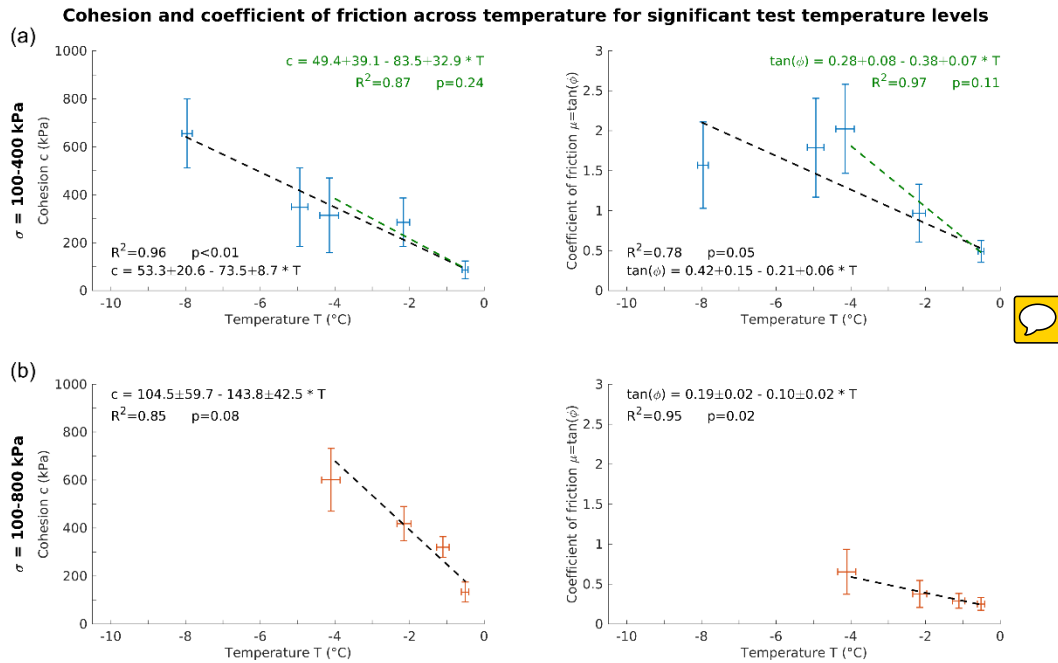
Figure 8: Cohesion and friction of ice-filled rock joints as a function of temperature for significant temperature levels with a statistical significance level of p \leq 5\% . The crosses display the means and standard deviations of rock temperature and cohesion or friction, grouped by the tested temperature class. (a) Tests at normal stresses 100–400 kPa and temperatures -8 to -0.5 ^{\circ}\text{C} (blue crosses). (b) Tests at normal stresses 100–800 kPa and temperatures -4 to -0.5 ^{\circ}\text{C} (orange crosses). The dashed lines represent the linear regression functions, which were inversely weighted with the squared standard errors. The green regression lines in (a) refer to a temperature range from -4 to -0.5 ^{\circ}\text{C} .
