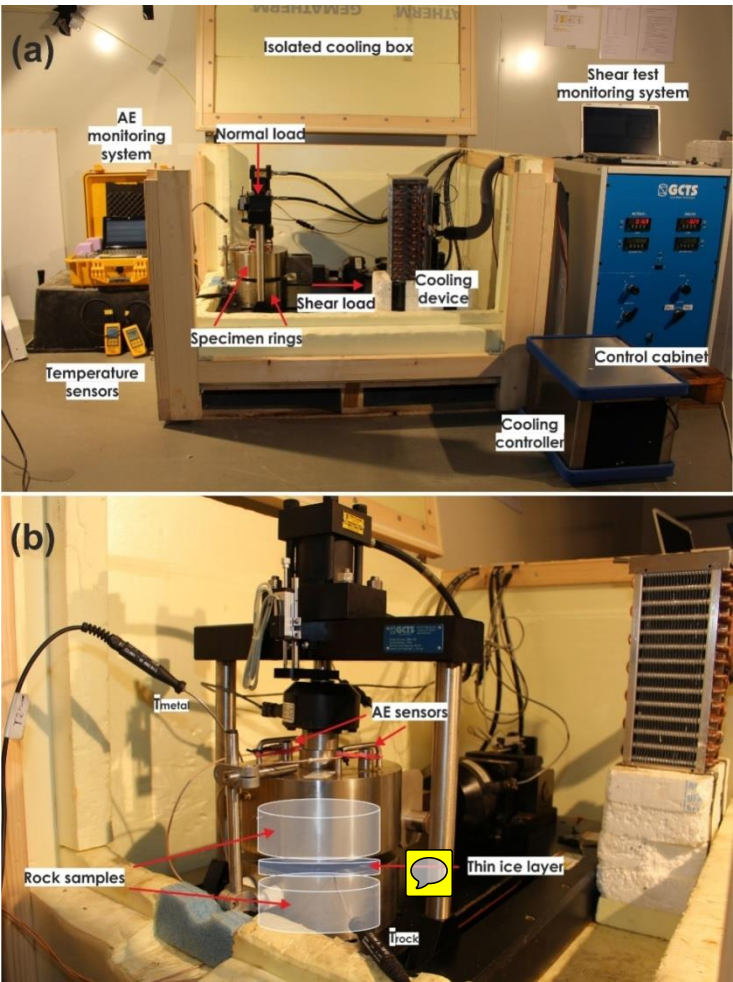
Figure 3: Experimental setup showing the laboratory shear machine, acoustic emission monitoring system, the cooling device and the cooling box.
