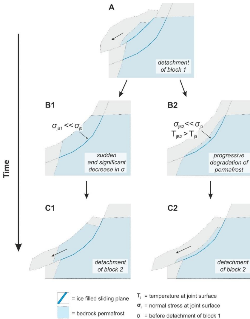
495 Figure 11: Progressive failure in a warming permafrost rock slope displaying thermal and normal stress conditions before and after detachment of a first slab. Both (B2) progressive thermal warming (i.e. permafrost degradation), but even faster (B1) sudden unloading can initiate failure.
