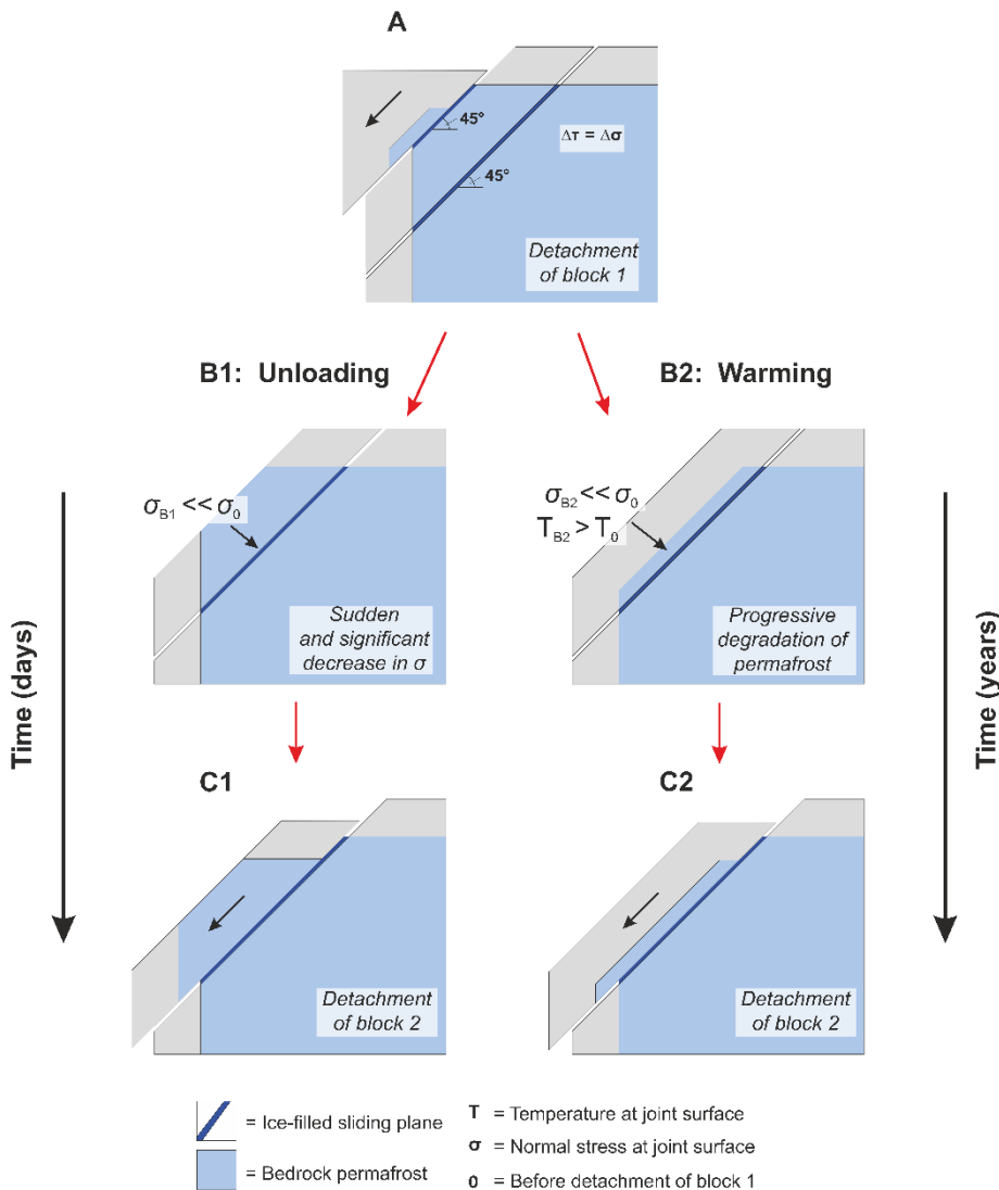
Figure 10: Progressive failure in a warming permafrost rock slope displaying thermal and normal stress conditions before and after detachment of a first slab. Both can initiate failure : (B2) Progressive thermal warming (i.e. permafrost degradation) occurs within years, but even faster -(B1) sudden unloading-can initiate failure develops, even faster within days.
