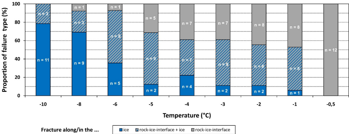
Figure 8: Proportions and absolute numbers of fracture types plotted at temperatures from -10 °C to -0.5 °C (for tests at 100–800 kPa). Failures inside the ice dominate at low temperatures whereas failure along rock-ice interfaces become more important close to 0 °C.
