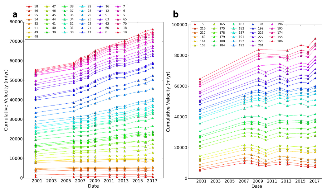
Figure 6. Summed speeds for collections of glaciers in (a) northwest and (b) southeast Greenland. The legend identifies individual glaciers using the glacier ids (numbers) used for the GIMP terminus position dataset (Moon and Joughin, 2008; Moon et al., 2015). Figure S1 shows the location of each numbered glacier. Because Jakobshavn represents such a large signal (Figure 3), we did not include it the northwest data. For a few glaciers, data is missing for some of the years plotted. In these cases, the stack is arranged with missing points on top so that data on either side bridge the gap.
