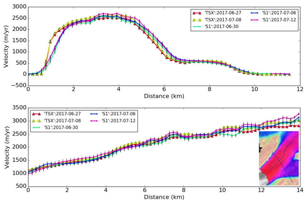
Figure 3. Profiles of speed from Sverdrup Glacier (see Figure 1 for location) along the (a) transverse and (b) longitudinal profiles shown in the inset. The speeds were calculated using individual TerraSAR-X (TSX) and Sentinel 1A/B (S1) pairs collected in early summer 2017.
