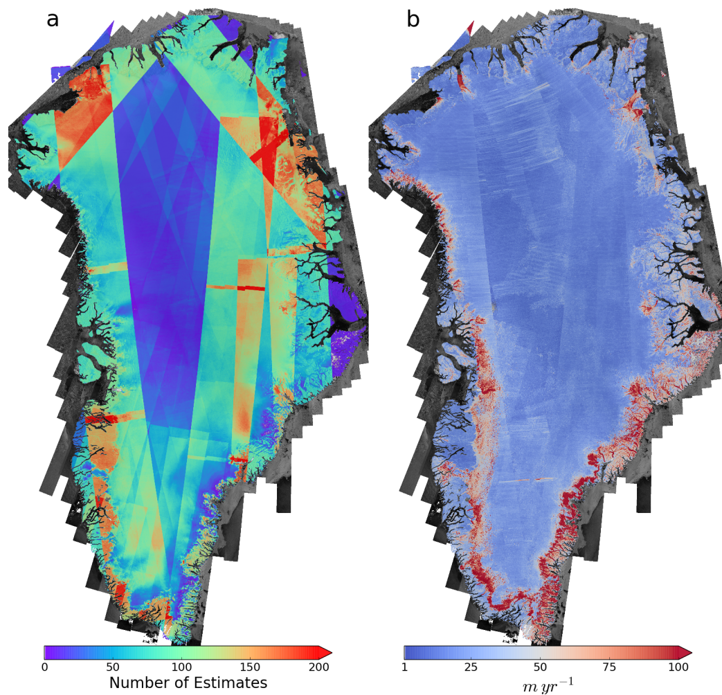
Figure 2. (a) Number of valid Sentinel 1A/B estimates made using data collected over the period from January 2015 to September 2017. (b) Combined standard deviation ( \sqrt{\sigma_{v_x}^2 + \sigma_{v_y}^2} ) of velocity estimates collected over the same period.
