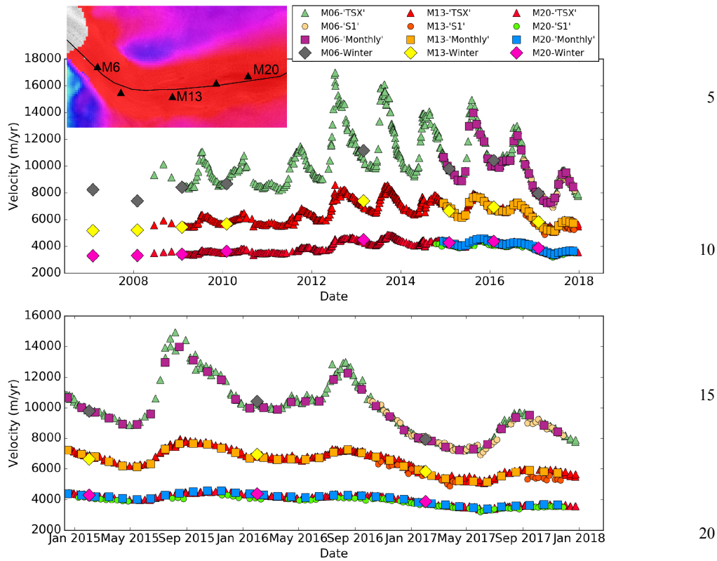
Figure 4. Speeds for Jakobshavn Isbrae at the points M6, M13, M20 shown in the inset over the periods from (a) 2007 to 2017 and (b) January 2015 to December 2017. Results show individual TerraSAR-X/TanDEM-X (triangles) and Sentinel 1A/B estimates (circles). Also shown are the aggregate monthly (squares) and winter (diamonds) products, which take advantage of all available data. For clarity we omitted the annual and quarterly products listed in Table 1. Error bars also are omitted because they are small relative to the plot marker size.
