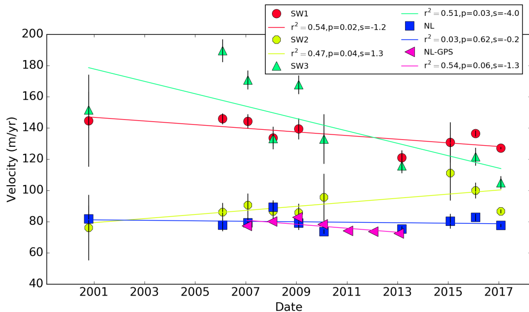
Figure 8. Winter velocities and corresponding trends for the points SW1–3 and NL (see Fig. 7 for location). Also shown are GPS derived speeds at NL (Stevens et al., 2016).
