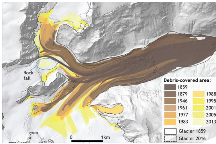
Figure 6: Current extent of debris cover and its evolution since 1859 (~the end of the LIA) together with the glacier outlines for LIA and 2016. Even though the glacier has retreated in the debris-covered region, debris covers more and more of the total glacier area.
