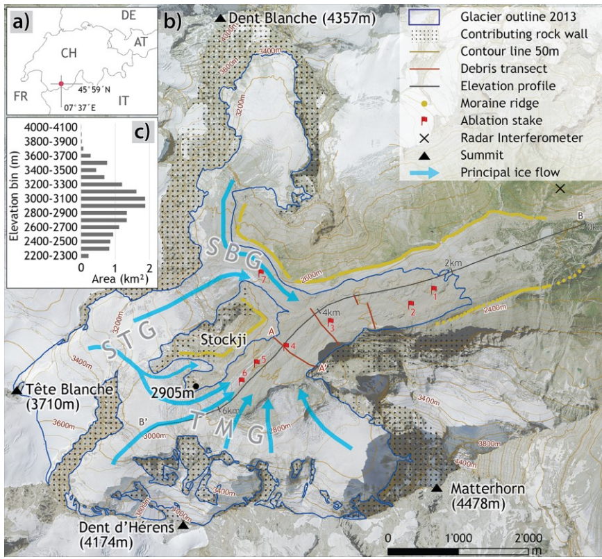
Figure 1: a): Geographical location. b): Zmuttgletscher, its topographical setting and different tributaries: SBG = Schönbielgletscher, STG = Stockjigletscher, TMG = Tiefmattengletscher. Background image: orthomosaic from aerial imagery by Swisstopo from 2013 (Swisstopo, 2010). c): Glacier hypsography in the year 2010.
