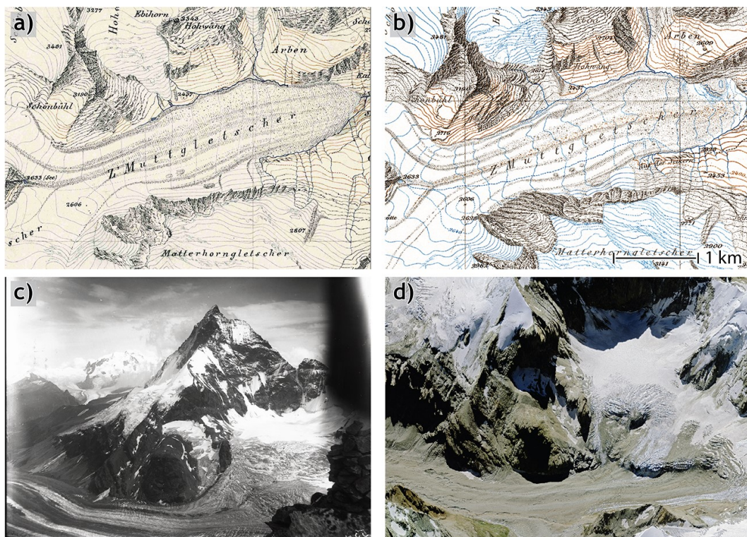
Figure 2: Example of mapped debris cover on (a) Dufour map, 1859, and (b) Siegfried map, 1879. c: parts of the tongue in 1894 in direction South-West (Reid, 1894; National Snow and Ice Data Center, 2002, updated 2015). d: similar extent as in c) in 2013 (Swisstopo, 2010).
