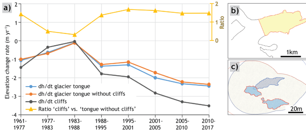
Figure 9: Influence of ice cliffs on total elevation change rate over the lowest area of the glacier tongue for eight time periods from 1961 to 2017. a): elevation change rate periods; b): area that was considered as 'tongue' for elevation change analysis; c): examples of ice cliffs of two different years (2005 = red; 2001 = blue), the corresponding borders of the 35 m buffer, and the overlapping area of this buffer (yellow, grey dotted area).
