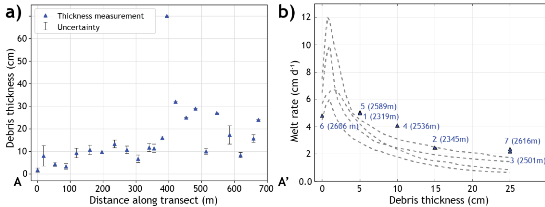
Figure 7: a): Debris thickness along the upper transect (Figure 1). Uncertainty bars represent the standard deviation of three measurements per location for depths <20 cm. b): Ablation of seven stakes over the time period 05.07.-22.08. 2017 (for locations see Figure 1). For comparison the curves of Rakhiot Glacier, Barpu Glacier, Kaskawalsch Glacier, and Isfallsgläciären (adapted from 15 Mattson et al., 1993).
