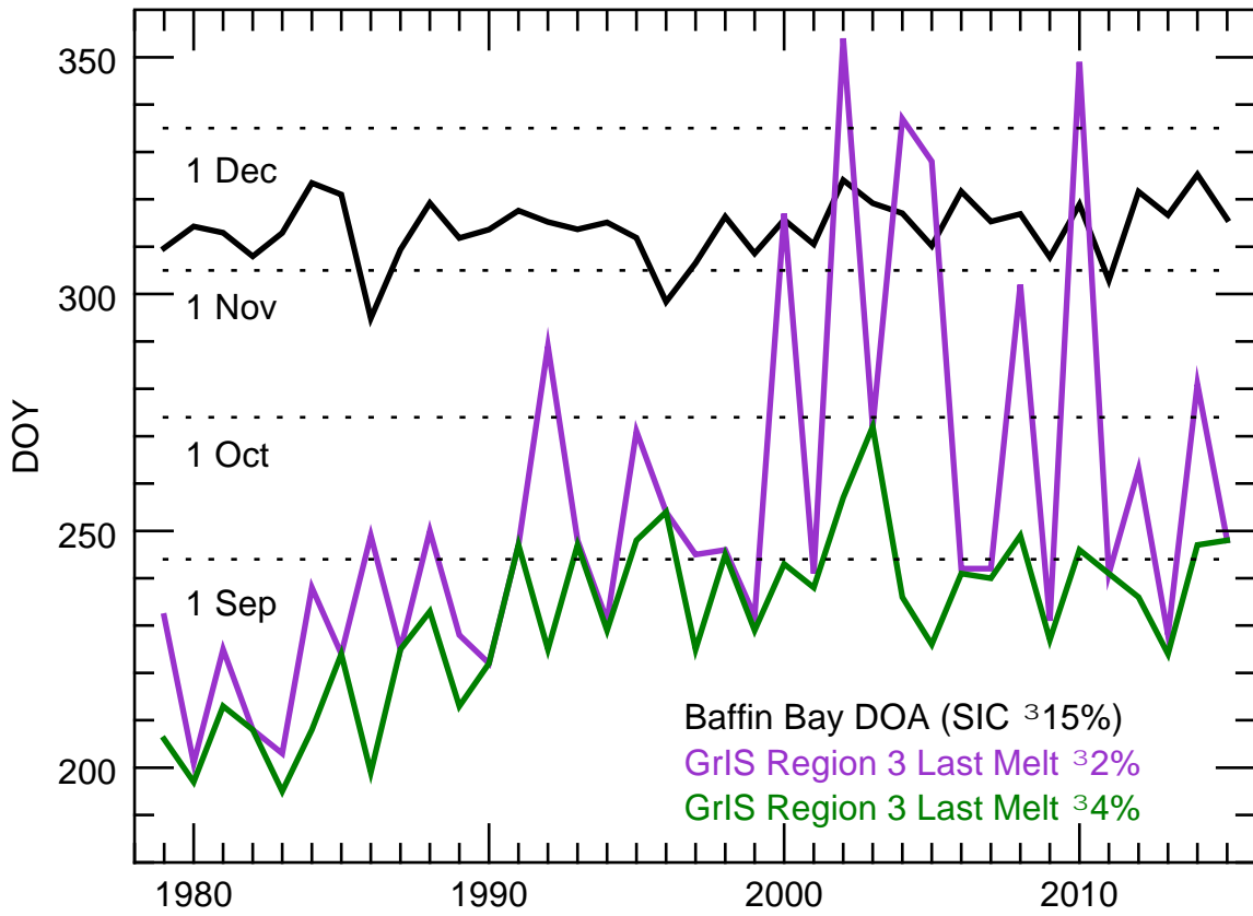
600 Figure 2. Passive microwave-derived time series, 1979-2015, of the Baffin Bay sea ice date of advance (DOA) and the date marking the beginning of the last 3-day period of at least 2% and 4% melt over Region 3 (see inset in Fig. 1 ) of the Greenland Ice Sheet (GrIS).
