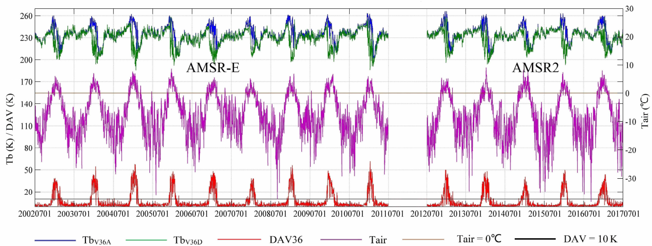
Figure 2. The comparison between T_{air} and satellite observations (AMSRE from 2002 to 2011 and AMSR2 from 2012 to 2017) at Zhongshan Station, including daily maximum T_{air} (purple line), T_{bv36A} (dark blue line), T_{bv36D} (dark green line) and DAV36 (red line); Brown and black lines represent T_{air} = 0^{\circ}C and DAV = 10 K .
