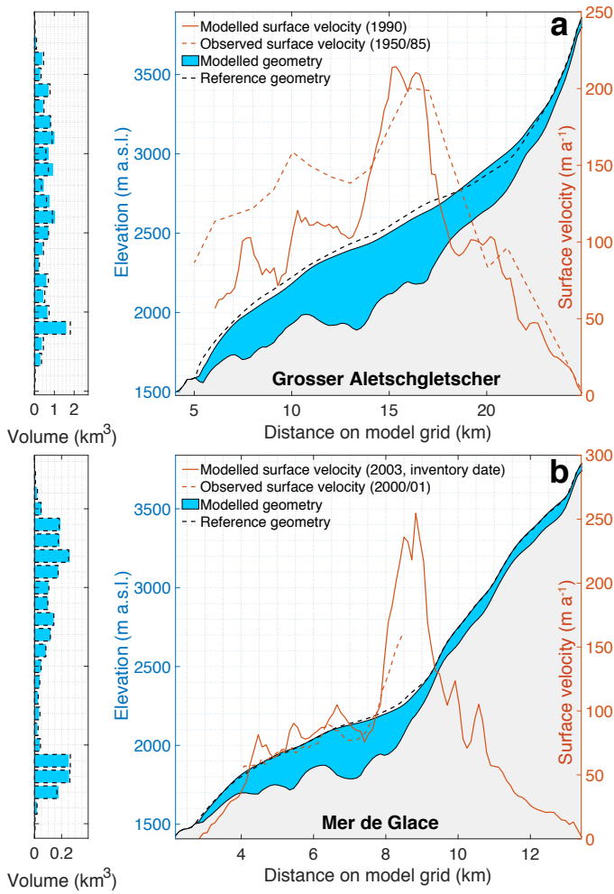
Fig. 5. Comparison between reference and modelled (i) glacier geometry, (ii) volume-elevation distribution and (iii) surface velocities for Grosser Aletschgletscher (a) and Mer de Glacier (b). Reference geometries and volume elevation distribution are at inventory date (2003) and based on Huss and Farinotti (2012). Observed surface velocities for Grosser Aletschgletscher are from Zoller (2010), and correspond to a 1950/1985 point averages, while observed velocities for the Mer de Glacier are derived from 2000/2001 SPOT imagery (Berthier and Vincent, 2012).
