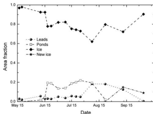
Figure 5. Average values of relative areas of ice, ponds, and leads from May 1998 through October 1998. Over 100 photos were analyzed for each flight.
