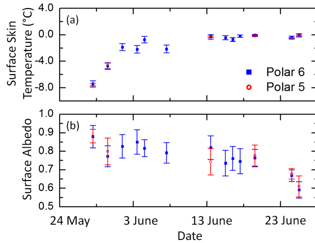
Figure 4. (a) Mean surface skin temperature over sea ice along flight tracks for selected days derived from KT19 measurements onboard of Polar 5 and Polar 6. (b) Mean Corresponding mean albedo of sea ice surface . The error bars give the standard deviation. The surface below the flight tracks was primarily snow covered sea ice, but the measurements also consider locations with open water.
