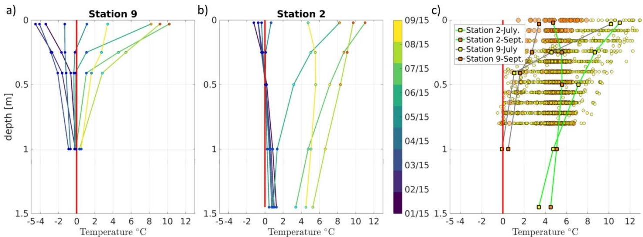
Figure 4: Temperature profile at Station (a) 9 and (b) 2 at every mid-month from January 15, 2017 to September 15, 2017). The zero Celsius degree line is in bright red. (c) Comparison of temperature measurements at Stations 2 and 9 (solid lines) with DTP measurements (circles) along transects A to E on July 17 (yellow) and along transects B and C on September 20 (orange).
