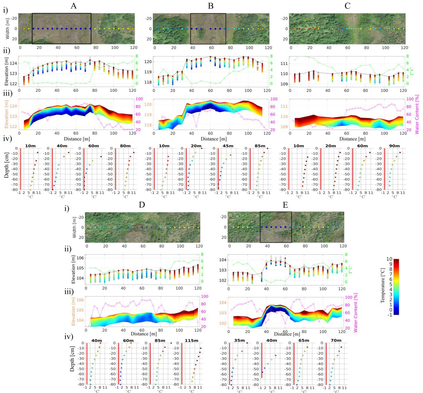
5 Figure 3: DTP data collected on July 17, 2017, along A-E transects. (i) Aerial view of the A-E transects in relative coordinate systems, overlain by temperature at 0.8 m depth and consequently identified near-surface permafrost areas (black rectangles), (ii) DTP temperature profiles and DTP temperature at 0.8 m depth (green line), (iii) Interpolated temperature map of the first 0.8 meter with topography and surface water content, and (iv) temperature profiles at selected locations along the transects.
