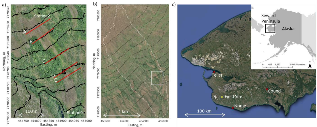
20 Figure 1: Location and general setting of the study area. a) Aerial view of the investigated site, which includes a hillslope and a flatter toe area. Tall shrubs are dark green, mosses are bright green, and graminoids and dwarf-shrub dominated areas are light brown. The RGB-mosaic is overlain with the location of the two long-term monitoring stations in this area, the location of transects surveyed in this study, and topographic isoline for every 5 m of elevation (in meter amsl.). b) Location of the investigated site (grey rectangle) in the Teller watershed. Topographic isoline for every 20 m of elevation. c) Location of the investigated field site on the South Seward Peninsula in Alaska.
