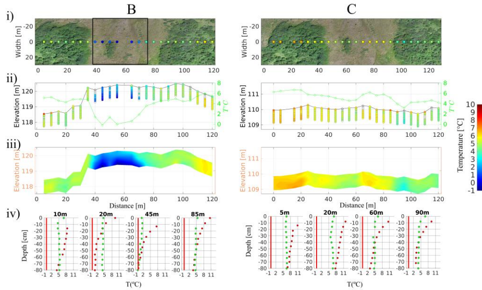
Figure 5: DTP data collected on September 20, 2017 along B and C transects. (i) Aerial view and identified near-surface permafrost area (from Figure 3) overlain by soil temperature at 0.8 m depth (green line), (ii) DTP temperature profiles and DTP temperature at 0.8 m depth, (iii) Interpolated temperature map of the first 0.8 meter with topography, and (iv) temperature profiles (green dots) at selected locations along the transects and compared to collocated temperature profiles acquired on July 17 (red dots, from Figure 3).
