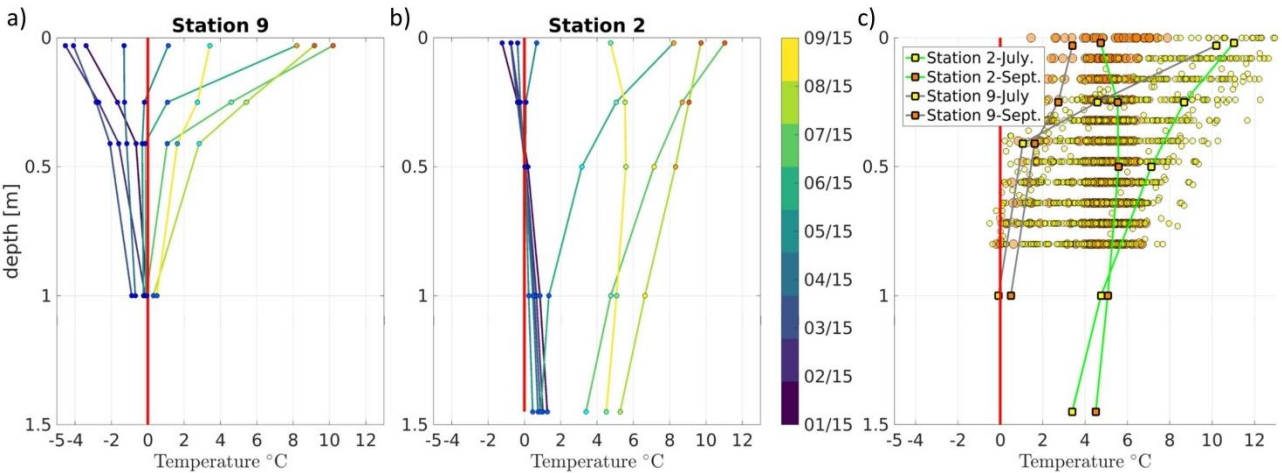
20 Figure 4: Temperature profile at Station (a) 9 and (b) 2 at every mid-month from January 15, 2017 to September 15, 2017). The zero Celsius degree line is in bright red. (c) Comparison of temperature measurements at Stations 2 and 9 (solid lines) with DTP measurements (circles) along transects A to E on July 17 (yellow) and along transects B and C on September 20 (orange).
