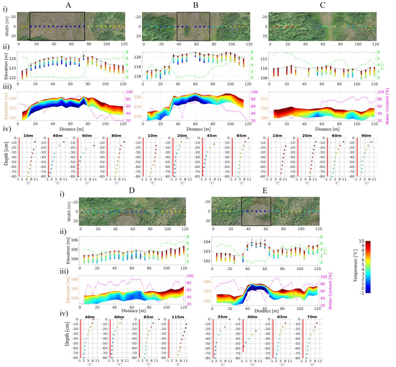
Figure 3: DTP data collected on July 17, 2017, along A-E transects. (i) Aerial view of the A-E transects in relative coordinate systems, overlain by temperature at 0.8 m depth and consequently identified near-surface permafrost areas (black rectangles), (ii) DTP temperature profiles and DTP temperature at 0.8 m depth (green line), (iii) Interpolated temperature map of the first 0.8 meter with topography and surface water content, and (iv) temperature profiles at selected locations along the transects.
