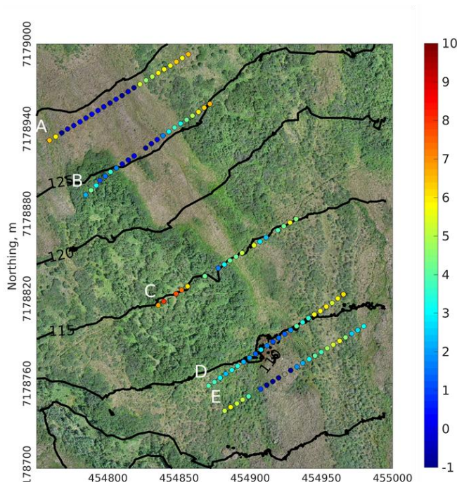
Figure 2: Temperatures at 0.8 m depth extracted from the DTP dataset collected on July 17 and topographic isolines for every 5 m of elevation (in meter amsl.).
