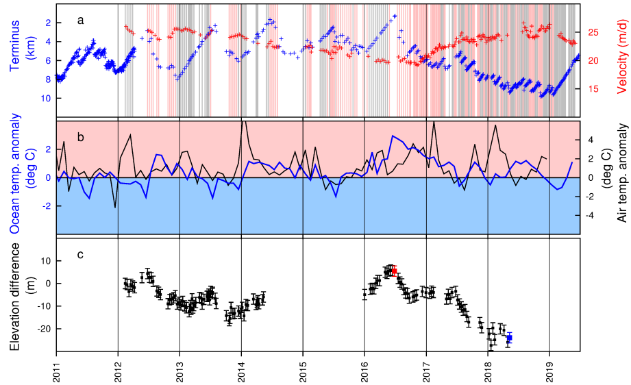
Figure 3. Time series plots. a) Front position and surface velocity (note the change in front position and velocity scales compared with Fig. 2a). The vertical bars mark dates when the feature-tracking metric indicated the presence (grey) or absence (pink) of a rigid mélange. b) 2 m air temperature anomaly for Aputiteeq, and Kangerdlugssuaq trough ocean potential temperature anomaly at 5 m depth averaged over the red box shown in Fig. 1 (blue). c) Cross-glacier mean surface elevation difference taken from the TanDEM-X DEMs, the error bars represent the relative accuracy of \pm 2.3 m. The elevations are an average across the transect marked in Fig. 6, and the differences are relative to the first DEM. The red and blue points mark the DEMs used for the surface elevation profiles plotted in Fig. 7.
