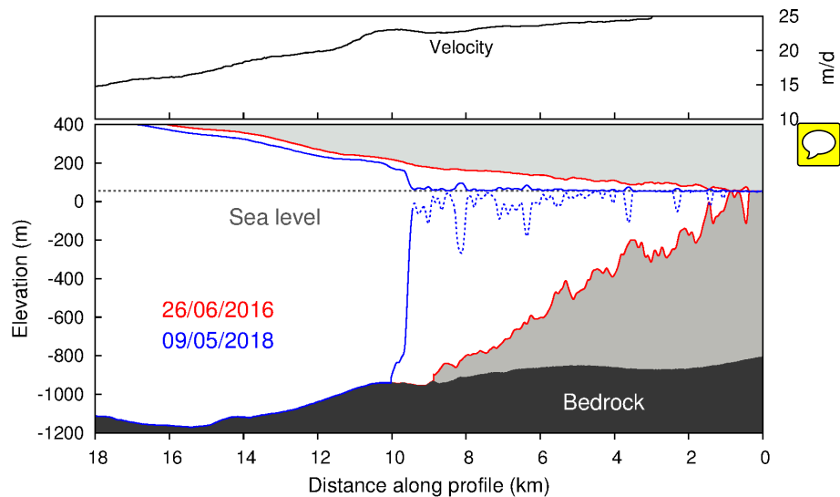
Figure 7. Surface elevation profiles for advanced (red) and retreated (blue) front positions, corresponding to the red and blue points plotted in Fig. 3c. The surface velocity profile is the result of feature tracking TerraSAR-X data from 29/05/2014 to 09/06/2014
