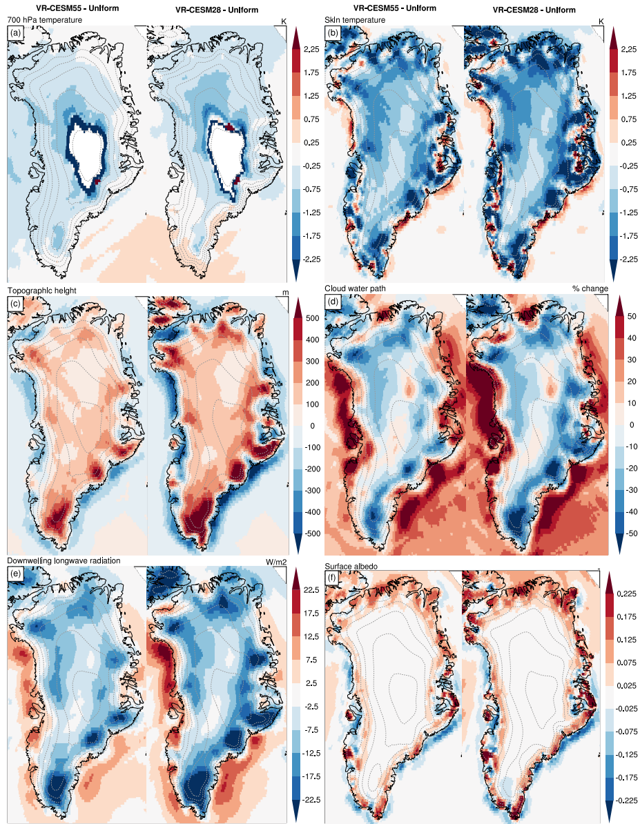
Figure 9. Summer (JJA) anomalies of atmospheric (CAM) variables over the period 1980-1999, relative to the coarse resolution reference simulation (Uniform CESM). Panel (a) 700 hPa air temperature [K], (b) radiative skin temperature [K], (c) CAM topographic height [m], (d) cloud water path [% change], (e) surface downwelling longwave radiation [ \text{W m}^{-2} ], (f) surface albedo [-]. Prior to subtraction, all data have been regridded to a common regular mesh of 0.25^\circ using bi-linear interpolation. Therefore, these anomalies should be interpreted with some caution since they contain interpolations errors. The "sinking oceans" in panel (c) are explained by the smoothing operator applied to CAM topography, the imprint of which is much wider at low resolution than it is at high resolution (cf. Figure 2 and Section 2.2).
