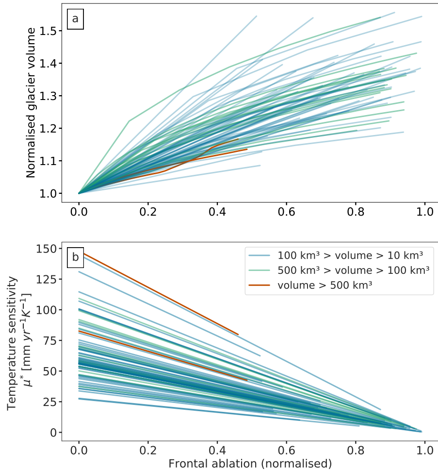
Figure 5. a: Normalised glacier volume and b: temperature sensitivity ( \mu^* ) of individual glaciers, as a function of the prescribed frontal ablation fluxes normalized normalised by the total accumulation over each glacier. The different colors represents different glacier classes.
