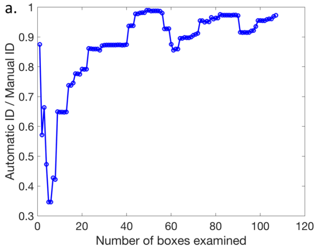
Figure 2: (a) The ratio of automatic iceberg detections to manual iceberg detections as a function of the cumulative number of test boxes counted (each box is 250 x 250 pixels). The total number of test boxes counted was 107. (b) Example of iceberg detection by algorithm. Gray ‘blotches’ not outlined in yellow are too small to be identified as icebergs, and are thus classified as mélange.
