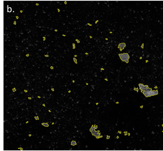
Figure 2: (a) The ratio of automatic iceberg detections to manual iceberg detections as a function of the cumulative number of test boxes counted (each box is 250 x 250 pixels). The total number of test boxes counted was 107. (b) Example of iceberg detection by algorithm. Gray ‘blotches’ not outlined in yellow are too small to be identified as icebergs, and are thus classified as mélange.
