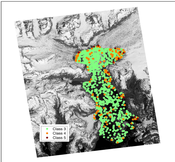
Figure 8: Location of large icebergs by centroid (May 06a). Icebergs in Class 3, Class 4, and Class 5 have waterline cross-sectional areas of 100 – 1,000 m 2 , 1,000 – 10,000 m 2 , and 10,000 – 100,000 m 2 respectively. The background satellite image was taken by WorldView 1 on June 10, 2013.
