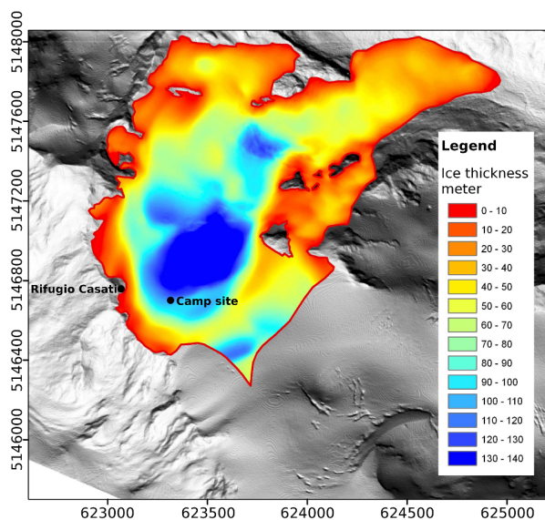
Figure 1. Extend and thickness map of the Langenferner glacier based on a modified figure in Stocker-Waldhuber (2010). The Casati hut and camp site of the field test are indicated. Coordinates are in UTM coordinates with east on the x-axis and north on the y-axis
