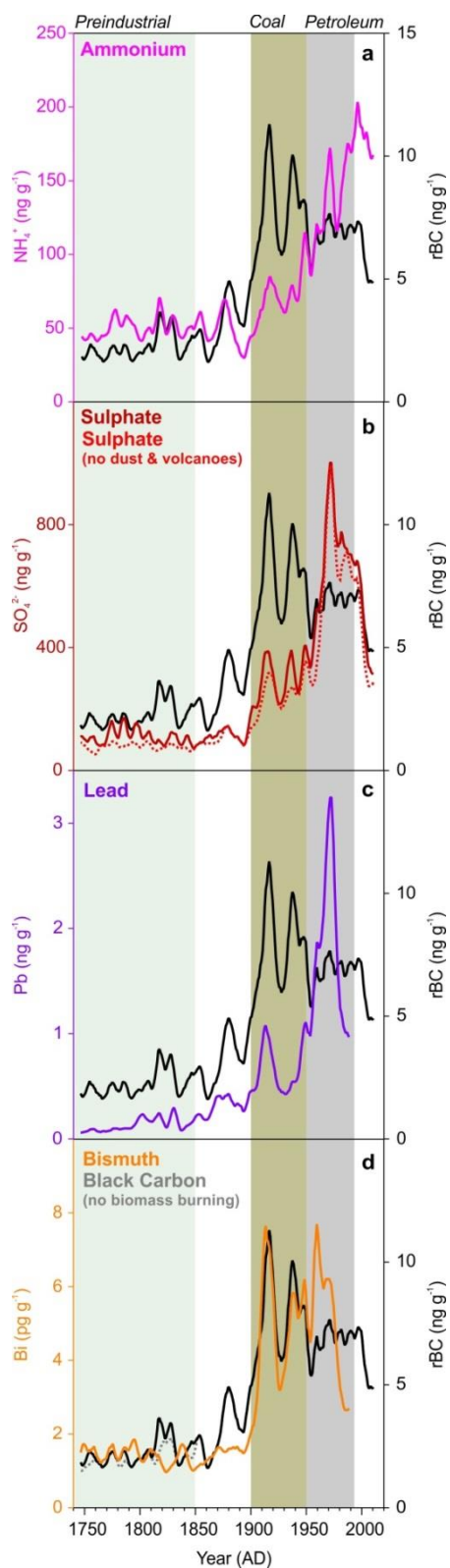
Figure 4: Colle Gnifetti rBC record (black) compared with a) ammonium (NH 4 + ), b) total sulphate (SO 4 2- ) and sulphate corrected for contributions from volcanic emissions and Saharan dust (dotted line), c) lead (Pb) and d) bismuth (Bi) together with rBC corrected for biomass burning contributions (BC no BB ; grey dotted line). All records are 11-yr filtered. Marked are time periods dominated by preindustrial emissions (1741-1850 AD), coal burning (1901-1950 AD) and petroleum burning emissions (1951-1993 AD), respectively.
