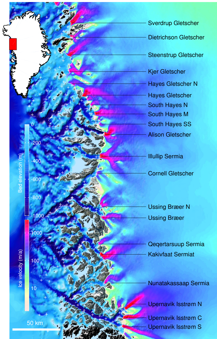
Figure 1. Ocean bathymetry (m, blue color scale) and ice velocity (m/a, Joughin et al., 2010) of Northwest Greenland. The white line shows the 2007 ice sheet extent, and white crosses indicate the locations of CTD data from NASA’s Oceans Melting Greenland campaign that are used to calibrate the thermal forcing.
