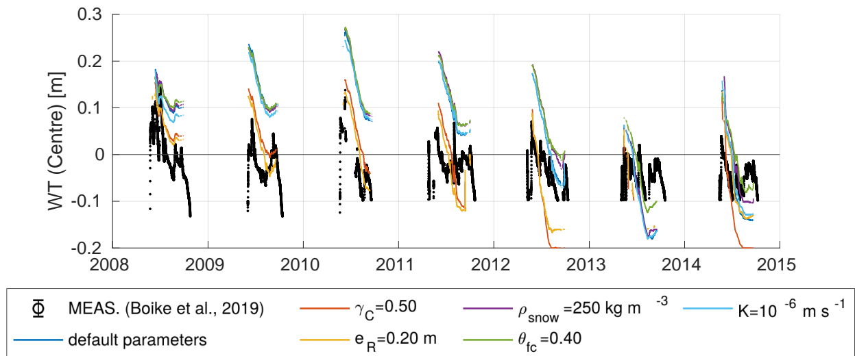
Figure 6. Modelled versus measured water tables (WTs) relative to the soil surface of a polygon centre for the 7-year period of the validation runs. The measured data are for a particular polygon centre on Samoylov Island described by Boike et al. (2019). Coloured lines correspond to the individually modelled WTs of the six validation runs (see Table 4 VALIDATION for default parameter values). Note that minimum WT measurements are limited to a level of -0.120 \text{ m} until 2009, and to -0.095 \text{ m} from 2010.
