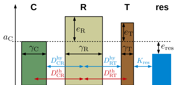
Figure 4. Setup of the coupled tiles (centres (C), rims (R), and troughs (T)) with parameters specifying the topology (reflected by areal fractions ( \gamma ), hydrological distances ( D^{hy} ), and thermal distances ( D^{th} )) and micro-topography (reflected by elevations ( e ) relative to the altitude of the centre tile ( a_C )) of the polygonal tundra landscape. Each tile was assigned a one-dimensional representation of the subsurface, for which a parallelized version of the CryoGrid3 Land Surface Model was used. Water can also be exchanged with the surrounding terrain, which is represented by a theoretical water reservoir (res) with a fixed water level ( e_{res} ) and a hydraulic conductivity ( K_{res} ). Subscripts denote the tile(s) the parameters are relating to.
