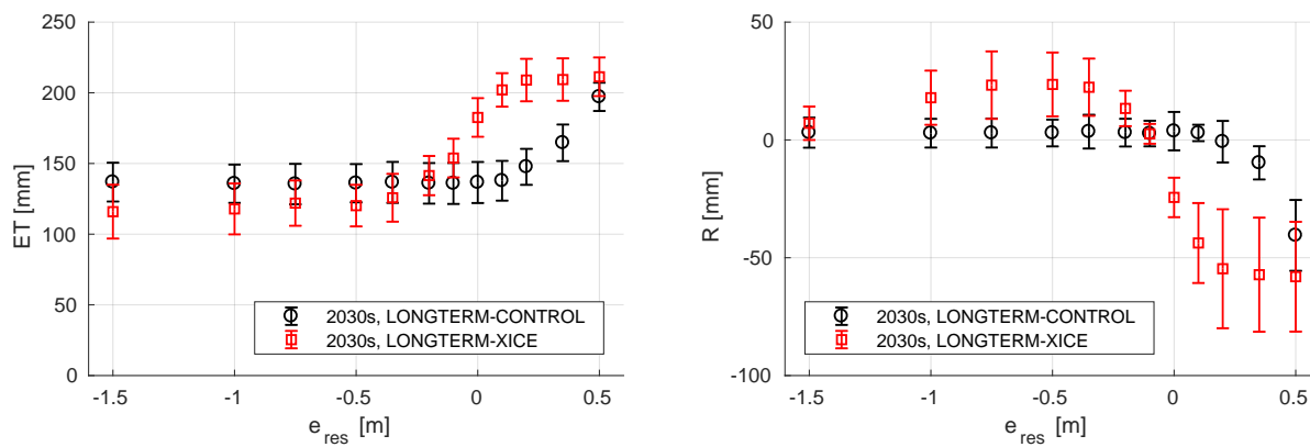
Figure 14. Changes to evapotranspiration (E, left panel) and external runoff (R, right panel) induced by the degradation of ice-wedges, for different hydrological conditions. Black markers show the means and standard deviations of the respective fluxes during the final 10 years of the simulation period (2030-2039) ignoring any ground subsidence (i.e., with disabled excess ice module). Red markers show the same for runs with enabled excess ice module, during which ice-wedge degradation occurred within the simulation period.
