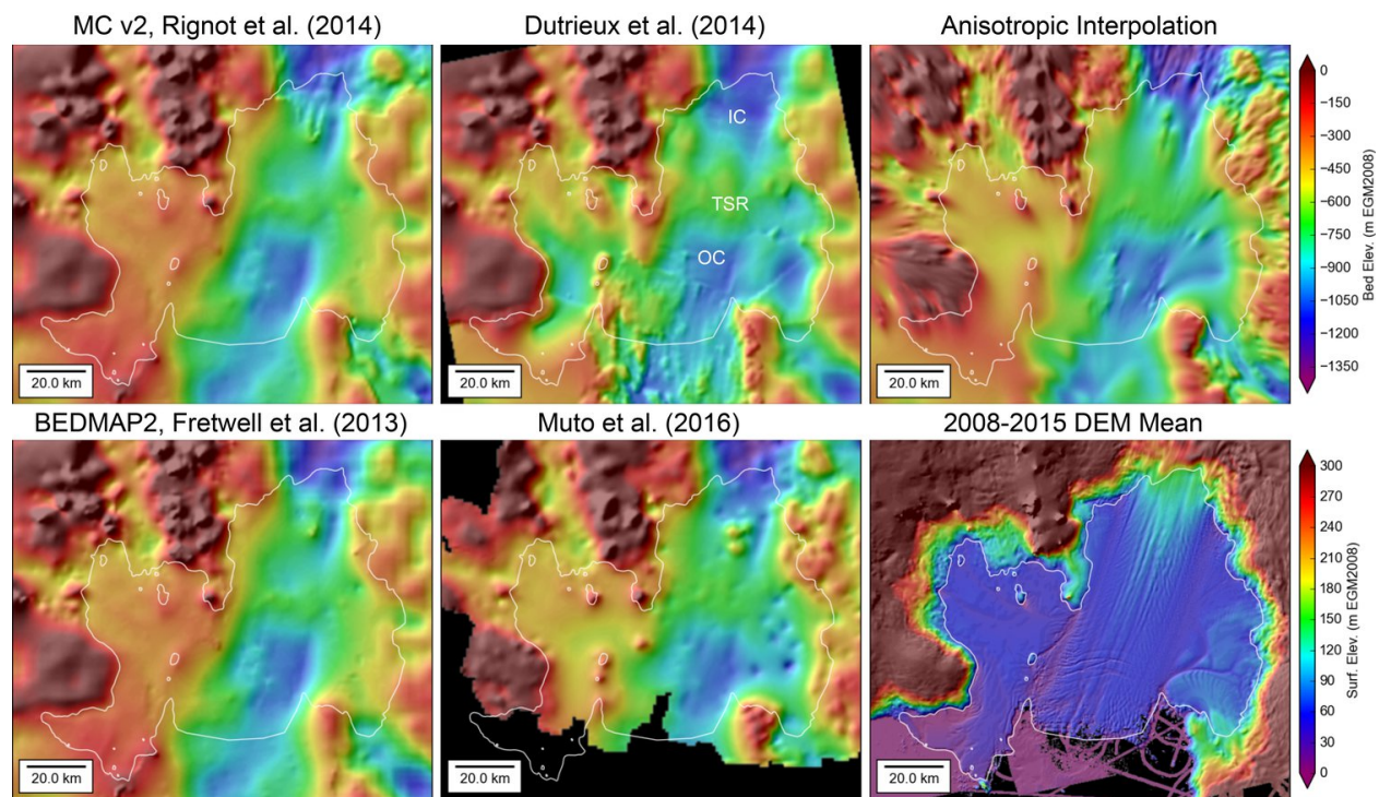
5 Figure S1: Comparison of available bathymetry/bed datasets for PIG with mean surface elevation for comparison. Top row, center column plot includes labels for "Transverse Seabed Ridge" (TSR), which separates the "Inner Cavity" (IC) and "Outer Cavity" (OC). Note significant differences in inner cavity bathymetry for the different datasets.
