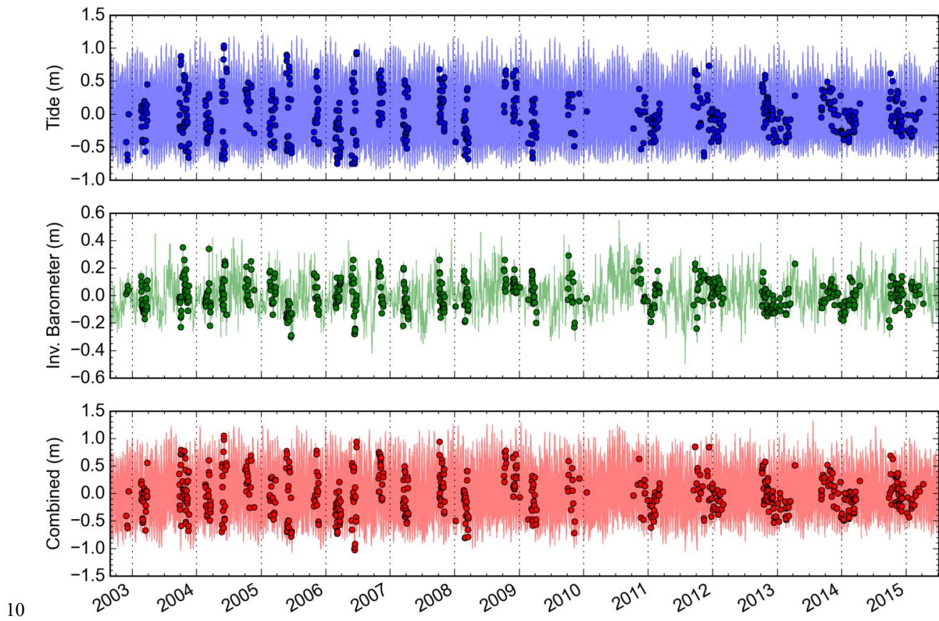
10 Figure S3: Magnitude of tide and inverse barometer corrections applied to timestamped DEM/altimetry elevation observations (points).
