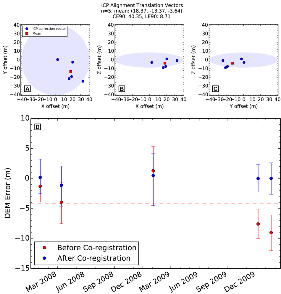
Figure S2: PIG SPIRIT DEM co-registration results. Refer to Error! Reference source not found. caption for details.
