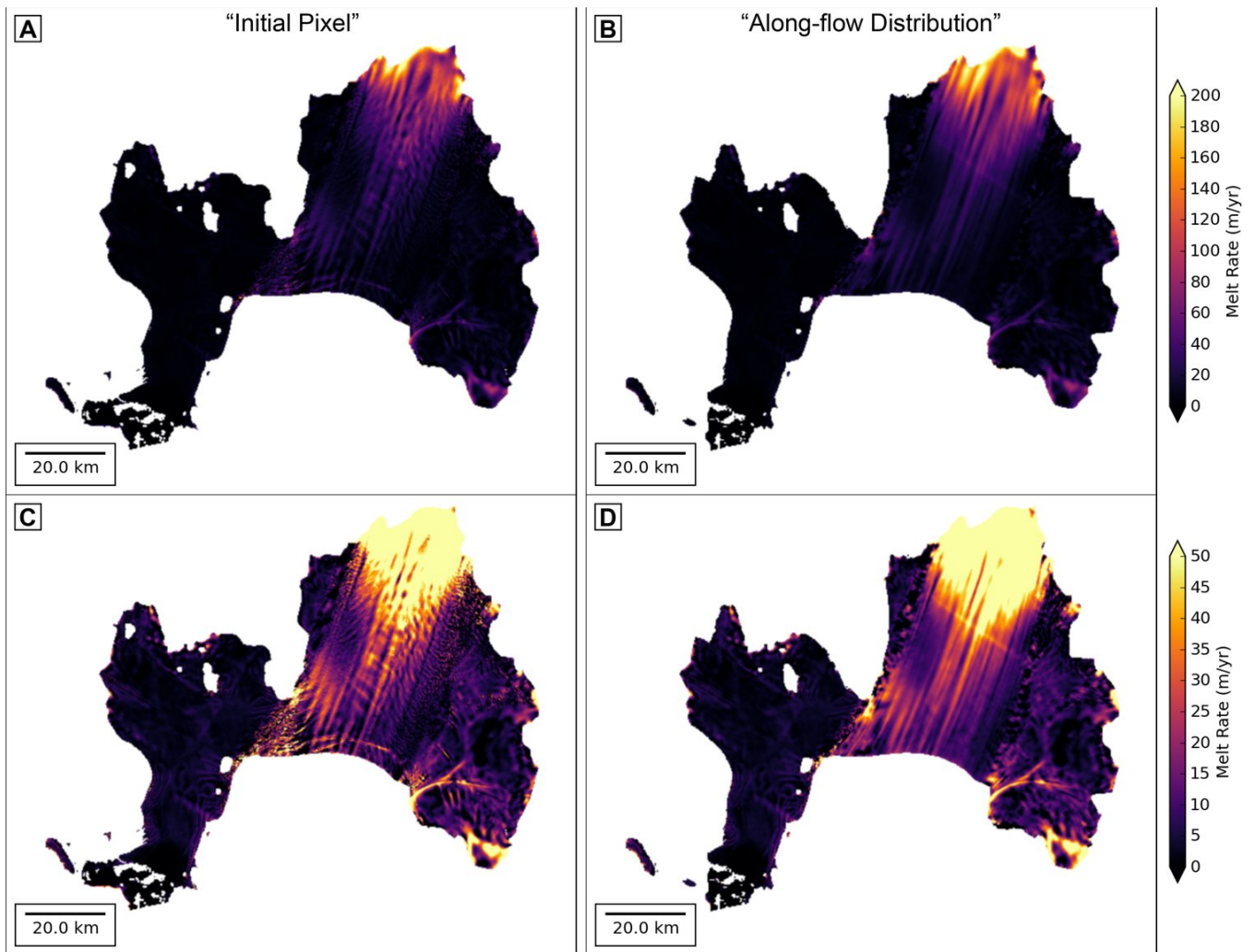
Figure S4: Mean 2008–2015 basal melt rates with different colorbar stretch.
