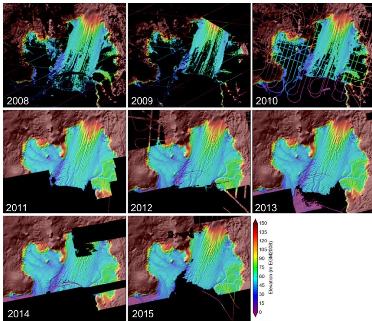
040 Figure 6: Annual DEM composites using all available elevation data. Primary DEM sources are SPIRIT (top row), and WorldView/GeoEye (middle and bottom rows).
