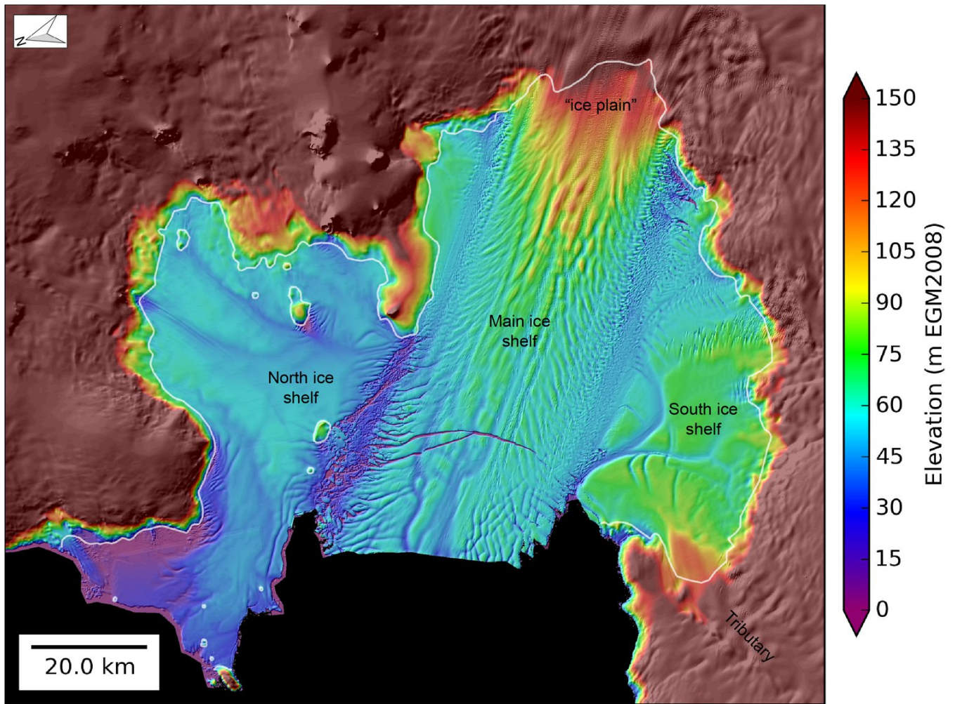
.015 Figure 3: October–December 2012 WorldView/GeoEye DEM mosaic of the PIG ice shelf. Labels show regions discussed in text: North ice shelf, South ice shelf, Main ice shelf, "ice plain", and fast-flowing South ice shelf tributary. White outline shows ~2011 grounding line. Elevation values are corrected surface height (Equation 1) above the EGM2008 geoid.
