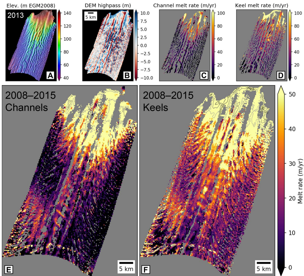
075 Figure 10: Relationship between km-scale surface ridge/trough (basal keel/channel) features and initial-pixel basal melt rates for main ice shelf. Top row shows example products from one 2-year period (2013–2015): A) 256-m DEM mosaic, B) km-scale surface anomalies after high-pass filter (surface ridges are blue, surface troughs are red), C) basal melt rates for channels (where DEM anomaly is <-1 m), D) basal melt rates for keels (where DEM anomaly is >1 m). Note relatively high basal melt rates over longitudinal basal channels at distances of \sim 4 – 15 km from the grounding line in C. The bottom row shows channel (E) and keel (F) melt rate composites generated using all available 2-year products during the full 2008 to 2015 period. Color stretch of 0–50 m/yr highlights differences over the outer ice shelf, where higher basal melt rates are observed on keels. See Figure S5 for additional details.
