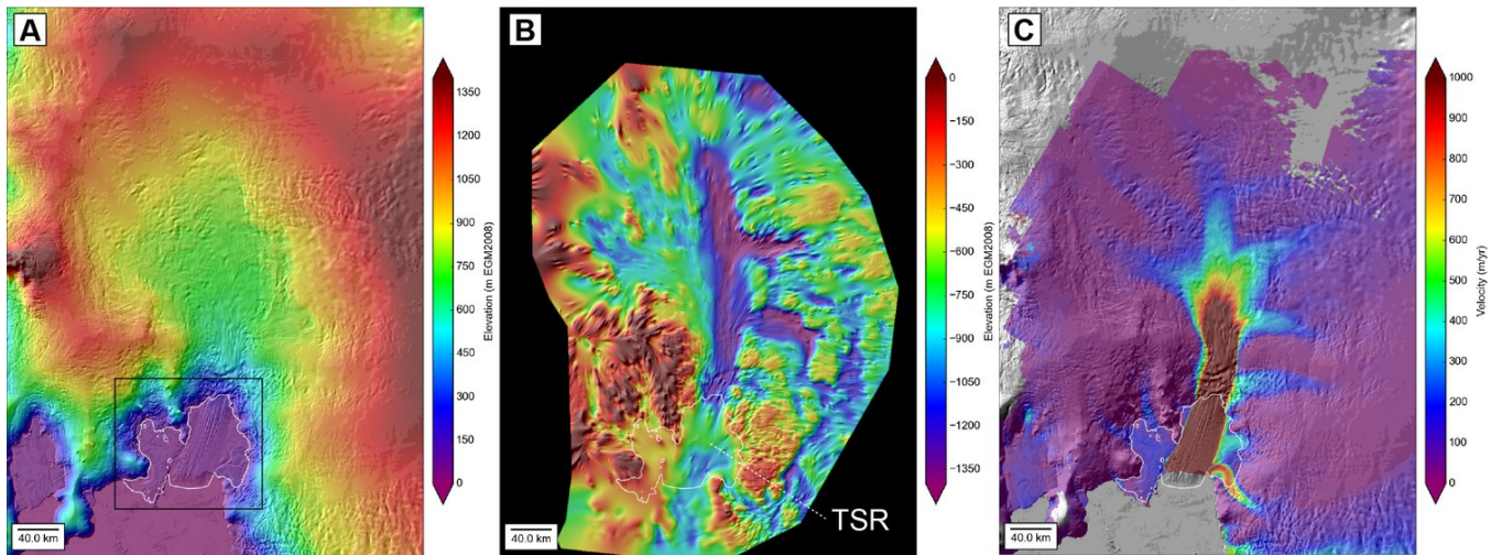
010 Figure 2: Context for the PIG catchment: A) High-resolution WorldView/GeoEye DEM mosaic over Bedmap2 DEM. White outline shows PIG ice shelf and ~2011 grounding line. Black box shows location of Figure 3. B) Combined bed topography and bathymetry from anisotropic interpolation of radar-derived ice thickness and other sources (see Section 2.6). Note bedrock channels beneath main trunk and tributaries. Dotted white line shows location of transverse seabed ridge (TSR) in PIG ice shelf cavity (see Figure S1 for detailed bed intercomparison). C) Median 2006-2016 surface velocity magnitude with color ramp saturated at 1 km/yr to show detail over tributaries (see Figure 1 of Shean et al. (2017) for color ramp saturated at 4 km/yr).
