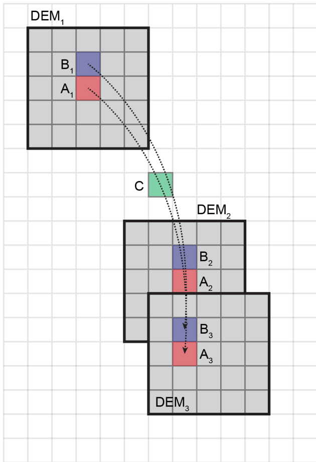
.045 Figure 7: Illustration of Lagrangian Dh/Dt calculation and basal melt rate distribution on a Eulerian grid (light gray). Three DEMs (medium gray) acquired at times t_1 , t_2 , and t_3 are resampled on this grid, with the same "features" A and B indicated as colored pixels. The position history for "particle" A is estimated using the velocity products described in Section 2.5, with paths indicated by dotted lines. Lagrangian Dh/Dt for A is calculated as (h_{A2}-h_{A1})/(t_2-t_1) . At each timestep along the path from A_1 to A_2 ( A_{12} ), we .050 estimate h (from observed Dh/Dt ), velocity divergence (from observed velocity time series), and the local flux divergence. Using Equations 10 and 12, the cumulative basal melt rate along the A_{12} path is estimated. This procedure is repeated for "particle" B and all other "particles" in DEM_1 that intersect DEM_2 . For the "along-flow distribution" approach, the cumulative basal melt rate for path A_{12} is assigned to each Eulerian grid cell along path A_{12} , including grid cell C. This assignment is repeated for path B_{12} and all .055 other paths for DEM_1 - DEM_2 particles, so that many basal melt rate values will be assigned to grid cell C. The median basal melt rate is calculated from all paths intersecting C. This median value at C (and all other grid cells with nonzero path count) are used to populate the along-flow distribution basal melt rate map for DEM_1 - DEM_2 . This process is repeated for DEM_1 - DEM_3 and all other .060 valid downstream DEM_1 - DEM_i combinations for the specified \sim 2 -year time period. The same process is then repeated for all initial DEM_i , and full ice shelf composites are generated as described in Section 3.6.1. For the "initial-pixel" approach, the cumulative basal melt rate for path A_{12} is assigned to cell A_1 . This process is repeated for the basal melt rate along path A_{13} and all other valid downstream DEM_i to estimate "initial-pixel" stack median basal melt rate for A_1 , and all other pixels in DEM_1 . This "initial-pixel" stack median process is repeated for all valid DEM_i , and these products are combined to create full ice shelf composites as described in Section 3.6.2.
