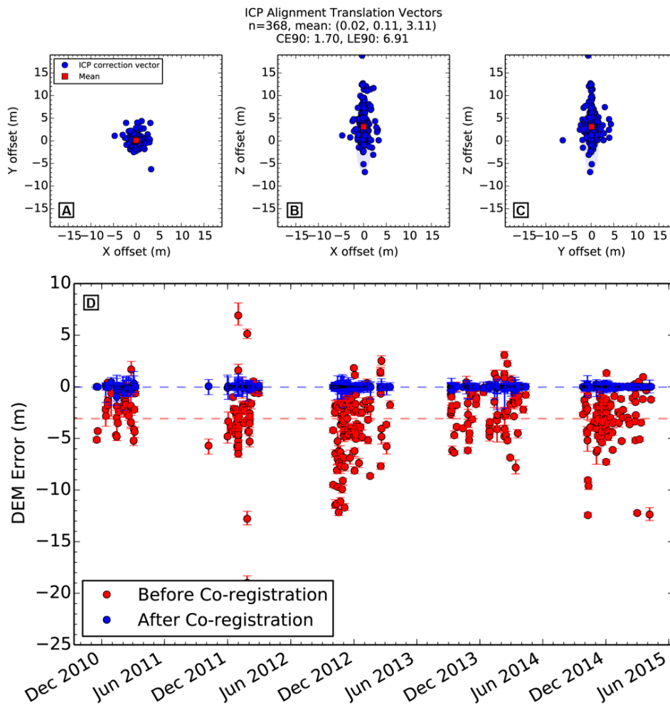
025 Figure 4: Co-registration results for 368 WorldView/GeoEye DEMs over PIG catchment (see Shean et al. (2016) for additional details). A-C) Iterative Closest Point (ICP) translation vector components required to co-register each DEM with filtered altimetry data. D) Median DEM error (DEM - altimetry) with error bars showing 16-84% spread for each DEM, before (red) and after (blue) co-registration. Horizontal dashed lines show mean error values. The 2011/2012 cross-track stereo DEMs display larger errors before co-registration. After co-registration, bias is removed and residual error spread for individual DEMs is typically <0.5–1 m, as summarized in Table 2.
