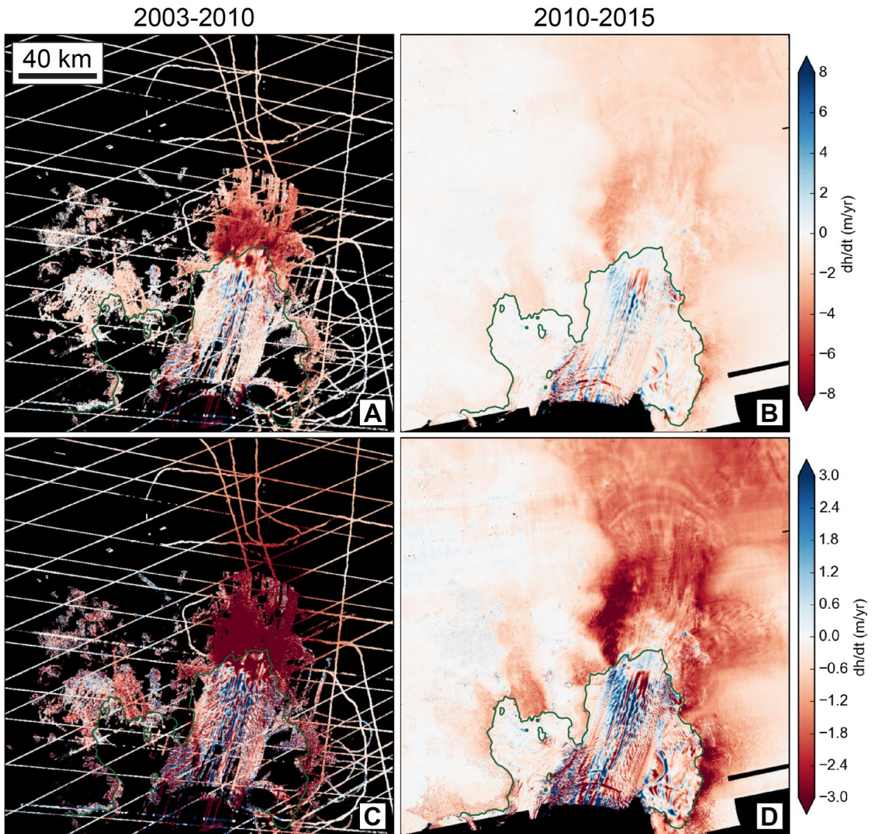
Figure 8: Long-term Eulerian dh/dt trends for the PIG ice shelf and lower catchment. A) 2003-2010 dh/dt from ICESat, ATM/LVIS airborne altimetry and SPIRIT DEMs. B) 2010-2015 dh/dt from WorldView/GeoEye DEMs, SPIRIT DEMs and ATM/LVIS airborne altimetry. C+D) Same data as in A+B, but with enhanced contrast stretch to bring out details over main trunk.
