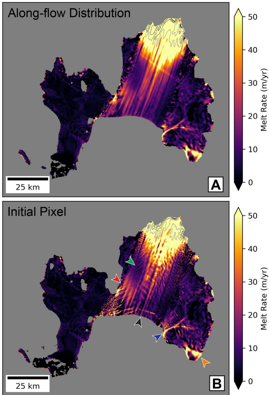
Figure 9: Comparison of mean 2008-2015 basal melt rate composites using: A) 2-year "along-flow distribution" and B) 2-year "initial-pixel" methods. Color ramp shows 0-50 m/yr stretch for basal melt rates, with additional grayscale contours at 100, 150, 200 and 250 m/yr near the grounding line. The transverse features along the outer ice shelf centerline in B are related to enhanced melt within and near depressions/rifts (Shean et al., 2017). The transverse mid-ice-shelf artifact in A is the result of a seam artifact in one of the TerraSAR-X velocity mosaics. Colored arrows show features discussed in the text.
