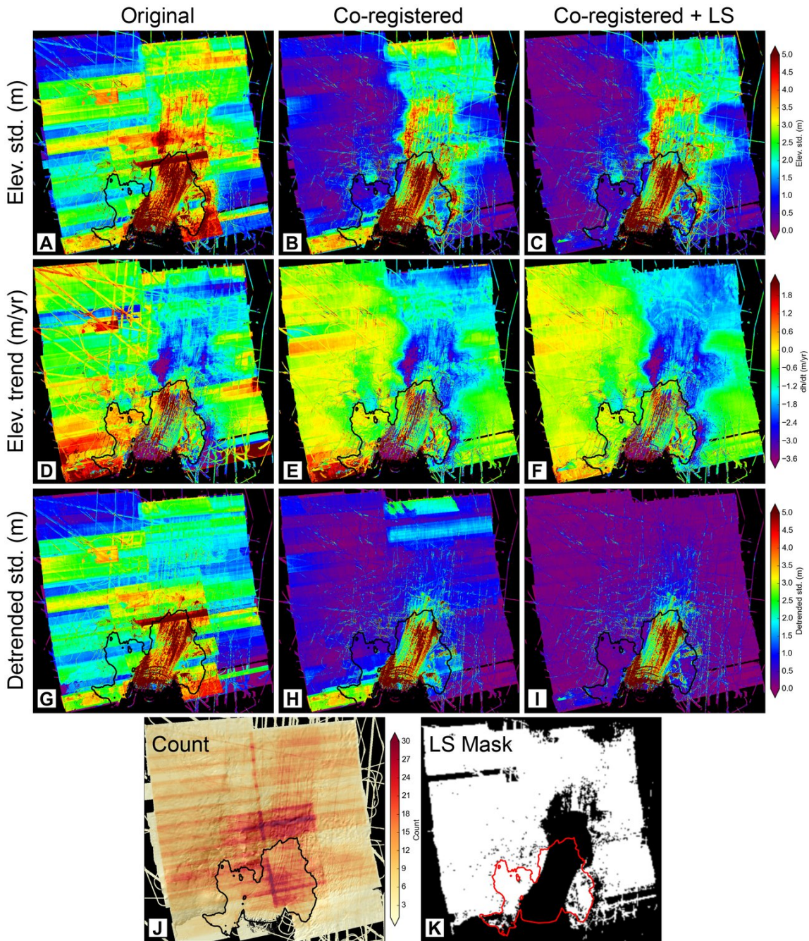
Figure 5: Statistics for 2010-2015 WorldView/GeoEye DEMs and available 2009-2015 ATM/LVIS altimetry data over the PIG study area. Top row (A-C) shows per-pixel elevation standard deviation, second row (D-F) shows per-pixel linear elevation trend, and third row (G-I) shows per-pixel standard deviation of residuals from linear regression. Left column (A,D,G) shows values for original DEM products before correction, center column (B,E,H) after ICP co-registration to filtered altimetry data, and right column (C,F,I) after least-squares optimization to correct residual DEM "tilt". Note overall improvement of final correction (right column). Bottom row shows per-pixel DEM count (J) and dynamic control surfaces (white) used during least-squares correction (K), as defined by criteria in Table 3.
